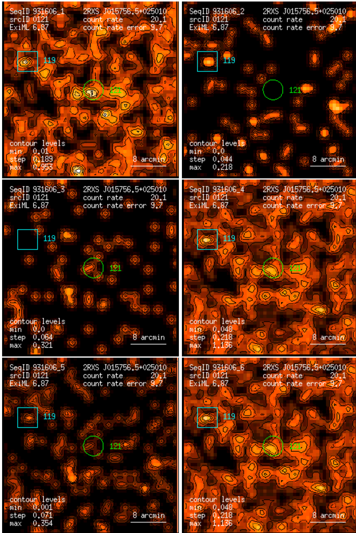
Figure 121: RASS 931606: detection 0121: band rate images, Gaussian filter: (1) PSPC channels 11 – 41, (2) 52 – 90, (3) 91 – 201, (4) 11 – 235, (5) 52 – 201, (6) 11 – 201. Broad band rates in counts/ks. Band rate contour levels in counts/ks/arcmin 2 .
