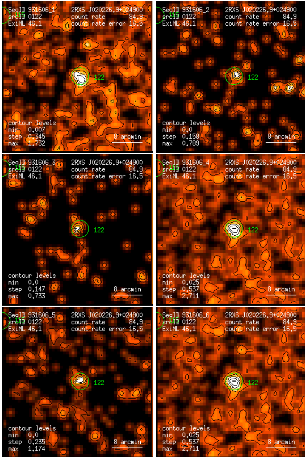
Figure 122: RASS 931606: detection 0122: band rate images, Gaussian filter: (1) PSPC channels 11 – 41, (2) 52 – 90, (3) 91 – 201, (4) 11 – 235, (5) 52 – 201, (6) 11 – 201. Broad band rates in counts/ks. Band rate contour levels in counts/ks/arcmin 2 .
