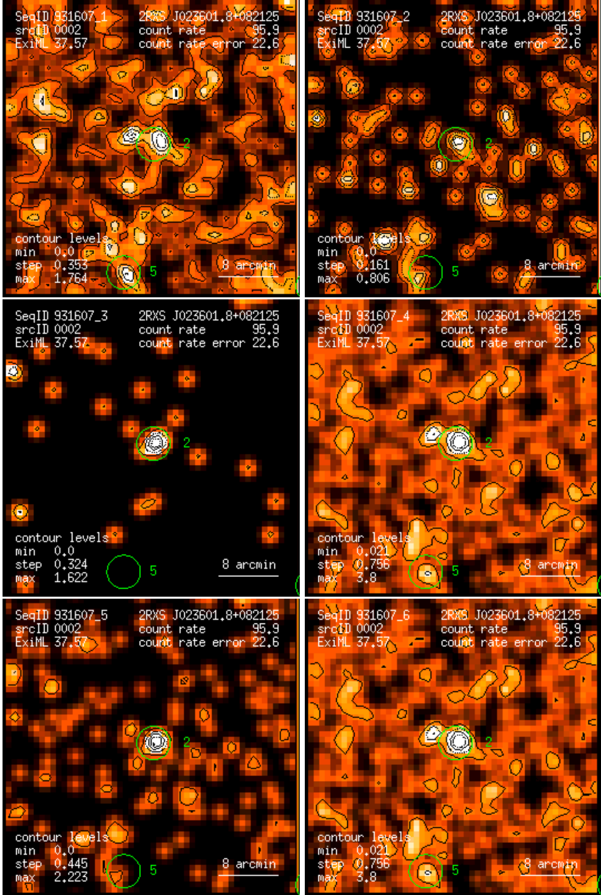
Figure 2: RASS 931607: detection 0002: band rate images, Gaussian filter: (1) PSPC channels 11 – 41, (2) 52 – 90, (3) 91 – 201, (4) 11 – 235, (5) 52 – 201, (6) 11 – 201. Broad band rates in counts/ks. Band rate contour levels in counts/ks/arcmin 2 .
