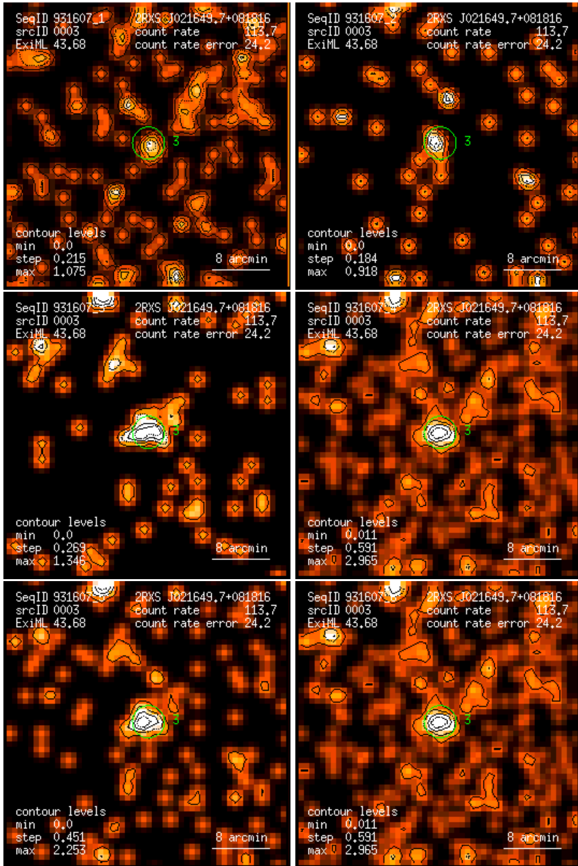
Figure 3: RASS 931607: detection 0003: band rate images, Gaussian filter: (1) PSPC channels 11 – 41, (2) 52 – 90, (3) 91 – 201, (4) 11 – 235, (5) 52 – 201, (6) 11 – 201. Broad band rates in counts/ks. Band rate contour levels in counts/ks/arcmin 2 .
