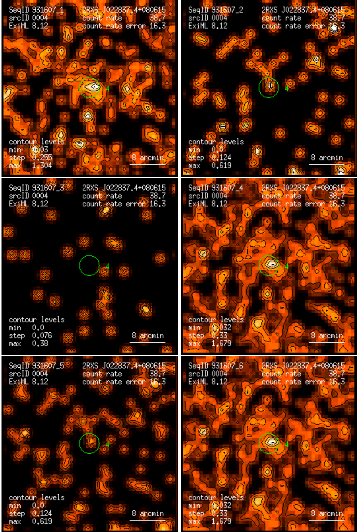
Figure 4: RASS 931607: detection 0004: band rate images, Gaussian filter: (1) PSPC channels 11 – 41, (2) 52 – 90, (3) 91 – 201, (4) 11 – 235, (5) 52 – 201, (6) 11 – 201. Broad band rates in counts/ks. Band rate contour levels in counts/ks/arcmin 2 .
