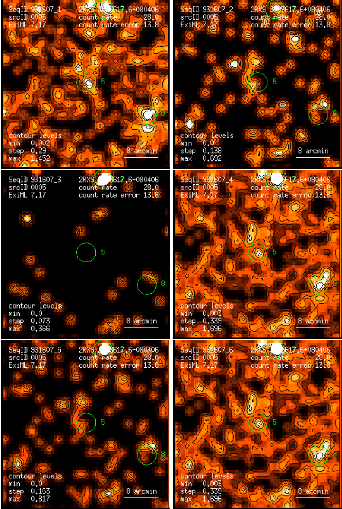
Figure 5: RASS 931607: detection 0005: band rate images, Gaussian filter: (1) PSPC channels 11 – 41, (2) 52 – 90, (3) 91 – 201, (4) 11 – 235, (5) 52 – 201, (6) 11 – 201. Broad band rates in counts/ks. Band rate contour levels in counts/ks/arcmin 2 .
