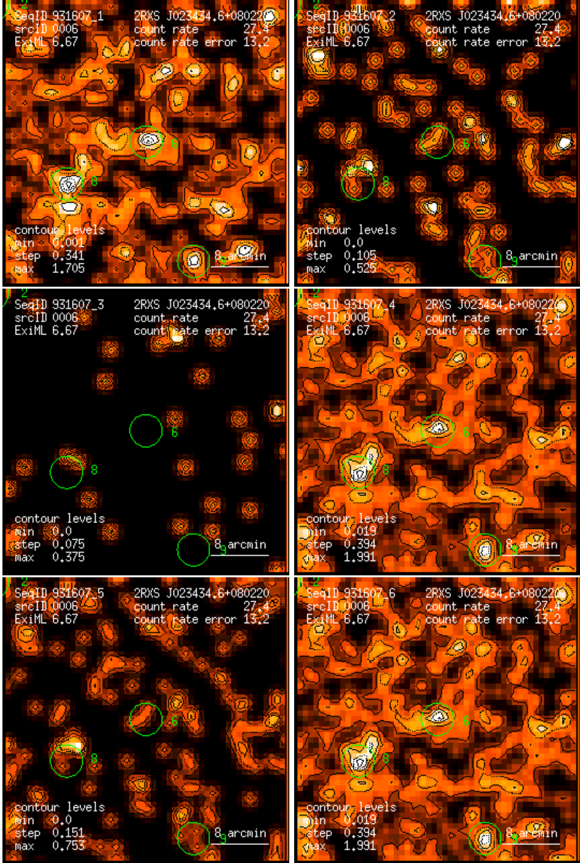
Figure 6: RASS 931607: detection 0006: band rate images, Gaussian filter: (1) PSPC channels 11 – 41, (2) 52 – 90, (3) 91 – 201, (4) 11 – 235, (5) 52 – 201, (6) 11 – 201. Broad band rates in counts/ks. Band rate contour levels in counts/ks/arcmin 2 .
