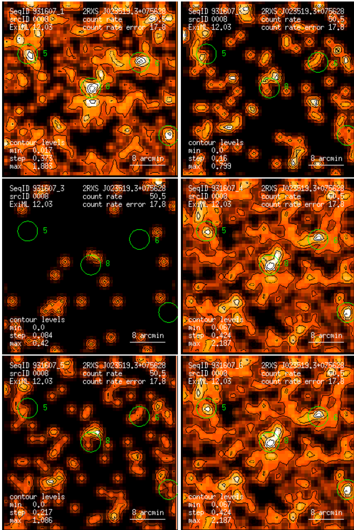
Figure 8: RASS 931607: detection 0008: band rate images, Gaussian filter: (1) PSPC channels 11 – 41, (2) 52 – 90, (3) 91 – 201, (4) 11 – 235, (5) 52 – 201, (6) 11 – 201. Broad band rates in counts/ks. Band rate contour levels in counts/ks/arcmin 2 .
