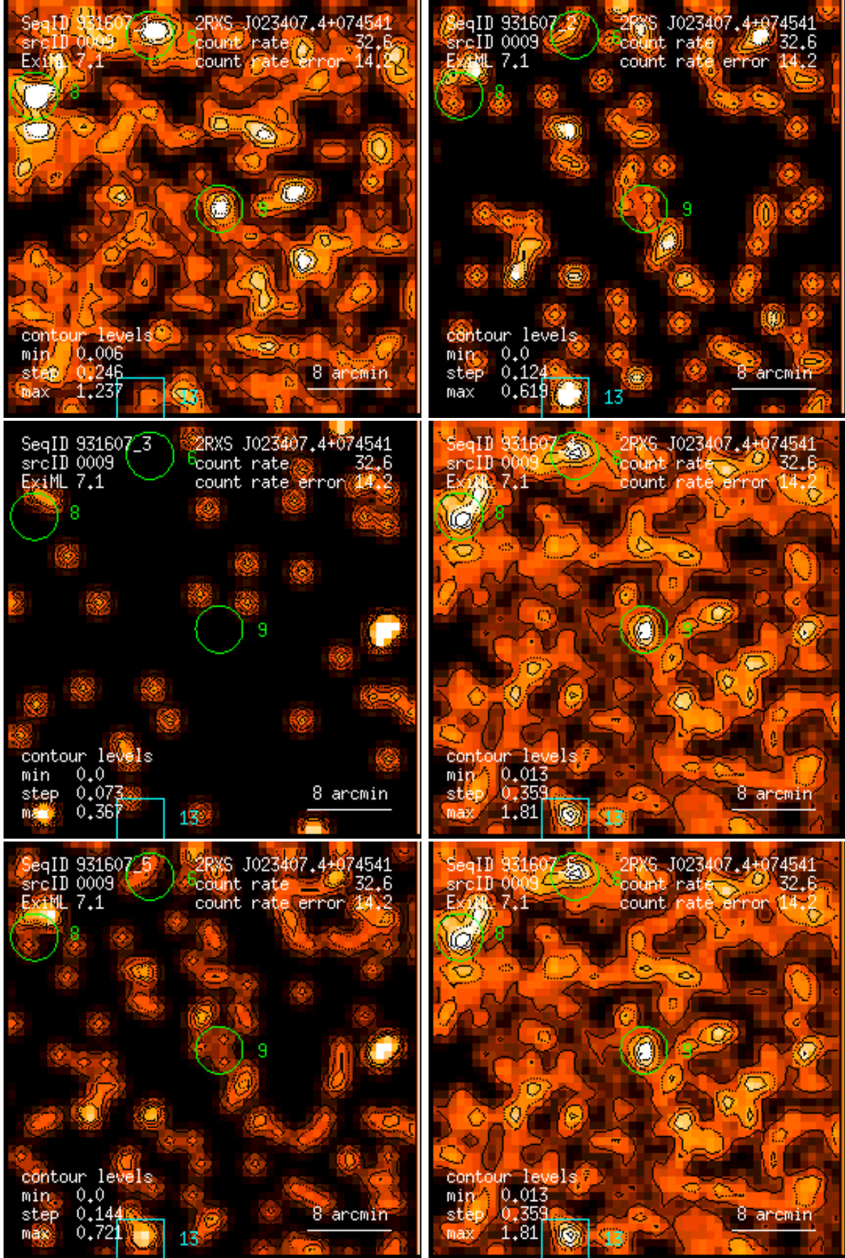
Figure 9: RASS 931607: detection 0009: band rate images, Gaussian filter: (1) PSPC channels 11 – 41, (2) 52 – 90, (3) 91 – 201, (4) 11 – 235, (5) 52 – 201, (6) 11 – 201. Broad band rates in counts/ks. Band rate contour levels in counts/ks/arcmin 2 .
