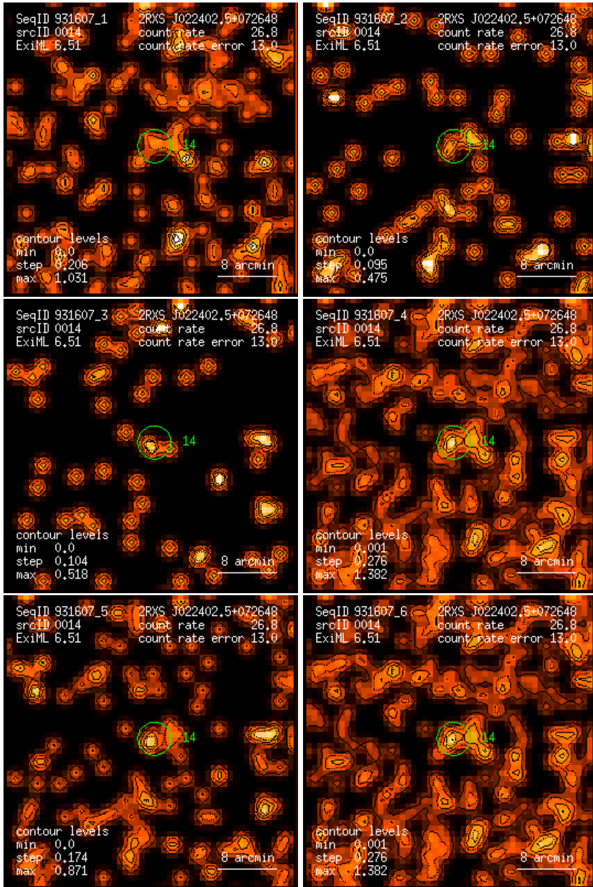
Figure 14: RASS 931607: detection 0014: band rate images, Gaussian filter: (1) PSPC channels 11 – 41, (2) 52 – 90, (3) 91 – 201, (4) 11 – 235, (5) 52 – 201, (6) 11 – 201. Broad band rates in counts/ks. Band rate contour levels in counts/ks/arcmin 2 .
