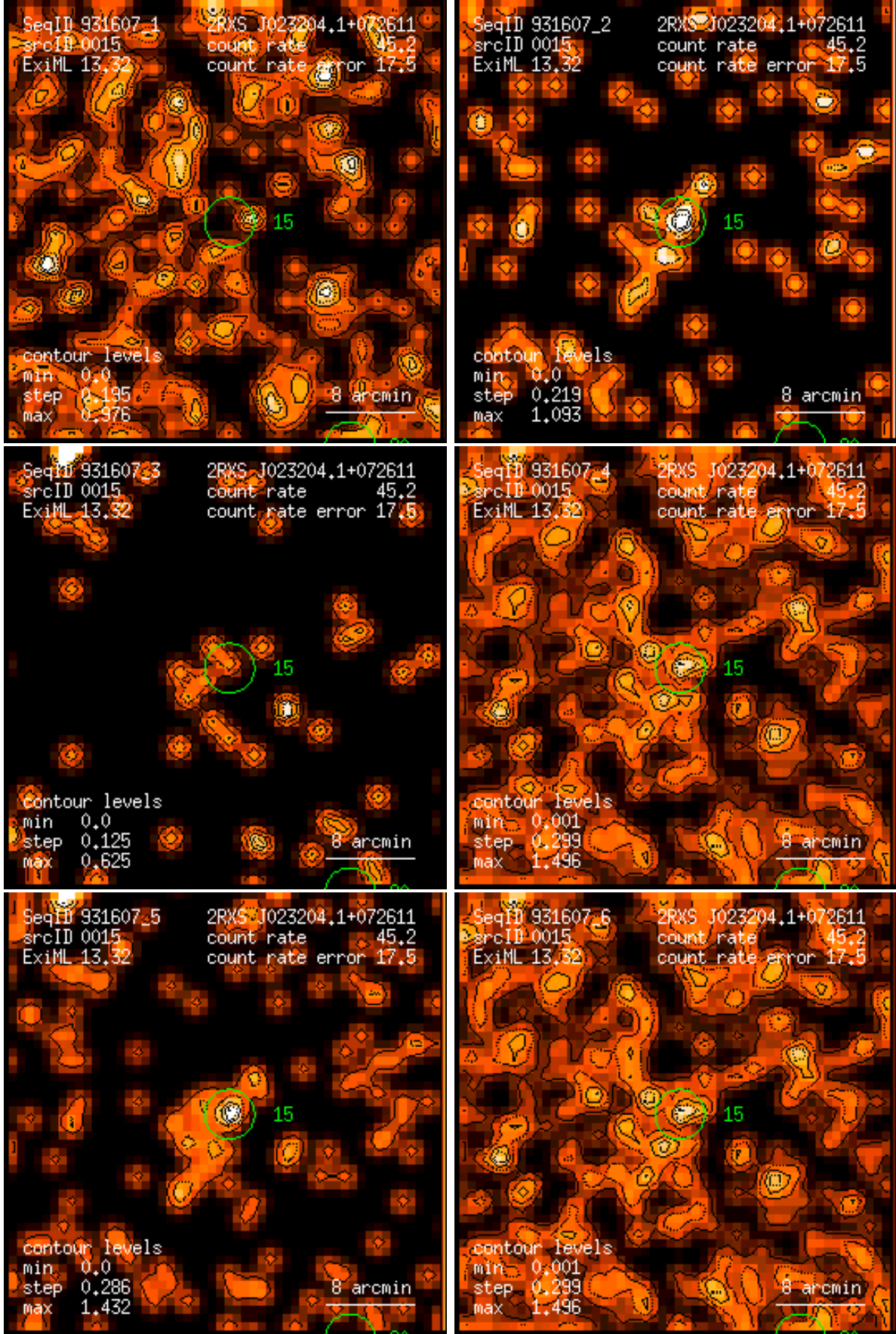
Figure 15: RASS 931607: detection 0015: band rate images, Gaussian filter: (1) PSPC channels 11 – 41, (2) 52 – 90, (3) 91 – 201, (4) 11 – 235, (5) 52 – 201, (6) 11 – 201. Broad band rates in counts/ks. Band rate contour levels in counts/ks/arcmin 2 .
