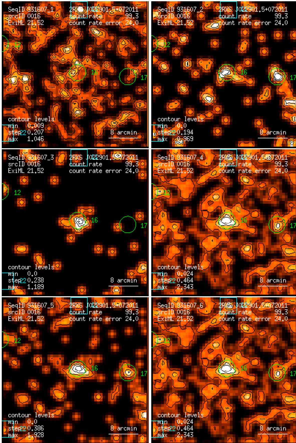
Figure 16: RASS 931607: detection 0016: band rate images, Gaussian filter: (1) PSPC channels 11 – 41, (2) 52 – 90, (3) 91 – 201, (4) 11 – 235, (5) 52 – 201, (6) 11 – 201. Broad band rates in counts/ks. Band rate contour levels in counts/ks/arcmin 2 .
