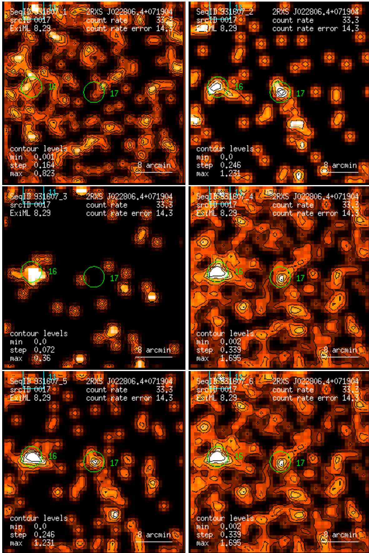
Figure 17: RASS 931607: detection 0017: band rate images, Gaussian filter: (1) PSPC channels 11 – 41, (2) 52 – 90, (3) 91 – 201, (4) 11 – 235, (5) 52 – 201, (6) 11 – 201. Broad band rates in counts/ks. Band rate contour levels in counts/ks/arcmin 2 .
