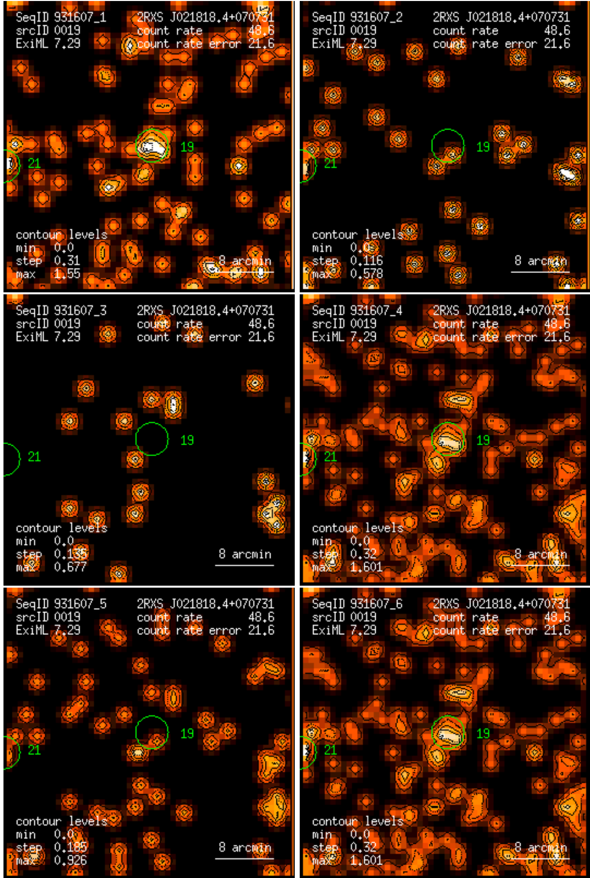
Figure 19: RASS 931607: detection 0019: band rate images, Gaussian filter: (1) PSPC channels 11 – 41, (2) 52 – 90, (3) 91 – 201, (4) 11 – 235, (5) 52 – 201, (6) 11 – 201. Broad band rates in counts/ks. Band rate contour levels in counts/ks/arcmin 2 .
