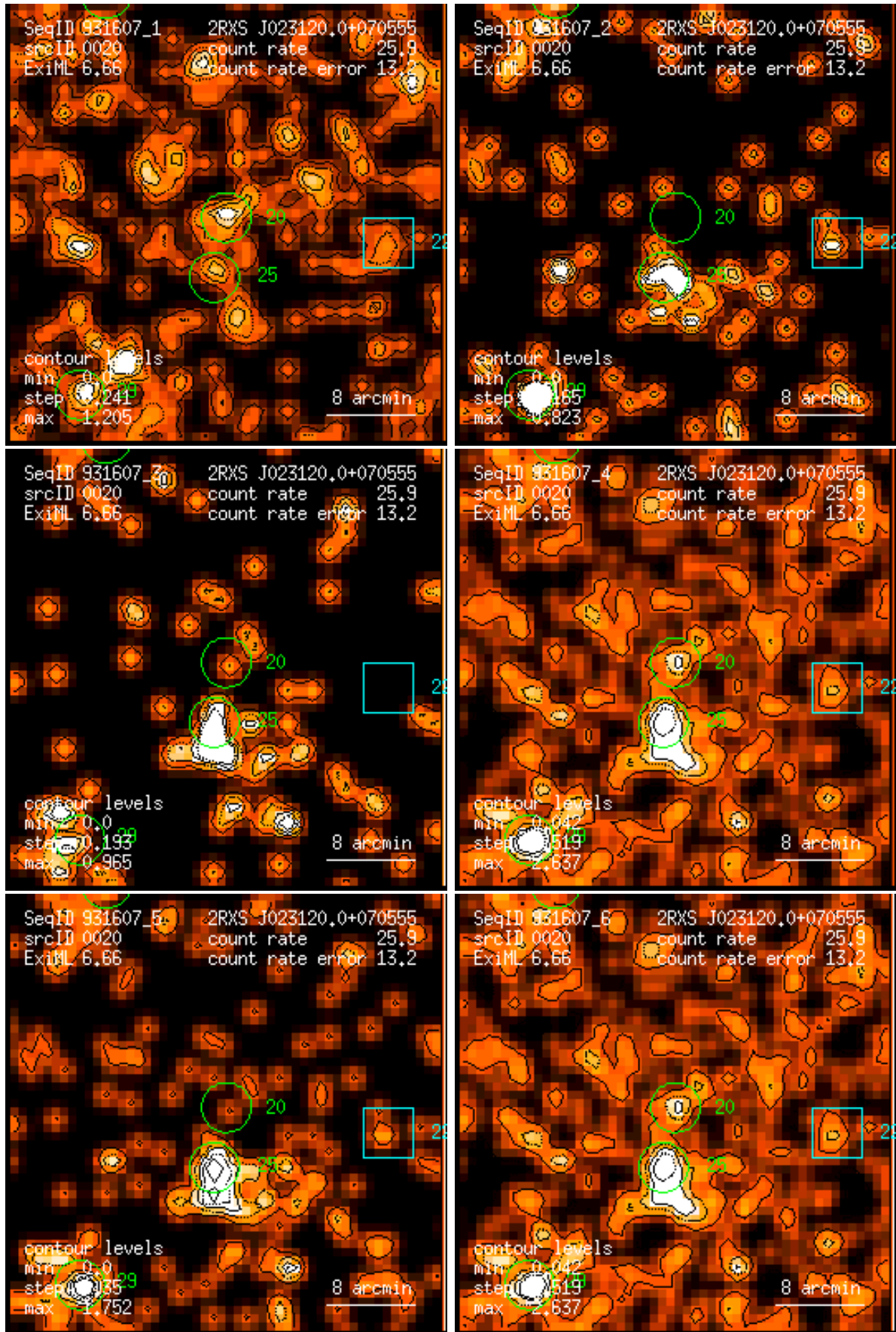
Figure 20: RASS 931607: detection 0020: band rate images, Gaussian filter: (1) PSPC channels 11 – 41, (2) 52 – 90, (3) 91 – 201, (4) 11 – 235, (5) 52 – 201, (6) 11 – 201. Broad band rates in counts/ks. Band rate contour levels in counts/ks/arcmin 2 .
