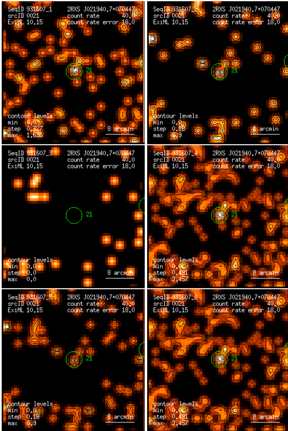
Figure 21: RASS 931607: detection 0021: band rate images, Gaussian filter: (1) PSPC channels 11 – 41, (2) 52 – 90, (3) 91 – 201, (4) 11 – 235, (5) 52 – 201, (6) 11 – 201. Broad band rates in counts/ks. Band rate contour levels in counts/ks/arcmin 2 .
