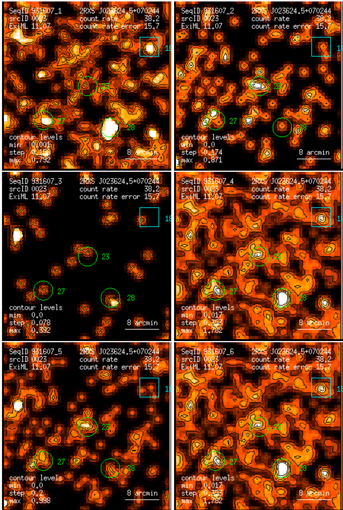
Figure 23: RASS 931607: detection 0023: band rate images, Gaussian filter: (1) PSPC channels 11 – 41, (2) 52 – 90, (3) 91 – 201, (4) 11 – 235, (5) 52 – 201, (6) 11 – 201. Broad band rates in counts/ks. Band rate contour levels in counts/ks/arcmin 2 .
