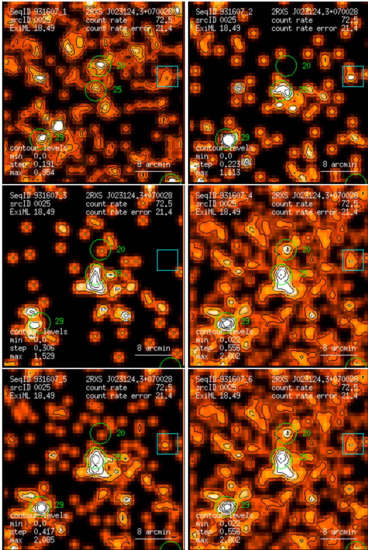
Figure 25: RASS 931607: detection 0025: band rate images, Gaussian filter: (1) PSPC channels 11 – 41, (2) 52 – 90, (3) 91 – 201, (4) 11 – 235, (5) 52 – 201, (6) 11 – 201. Broad band rates in counts/ks. Band rate contour levels in counts/ks/arcmin 2 .
