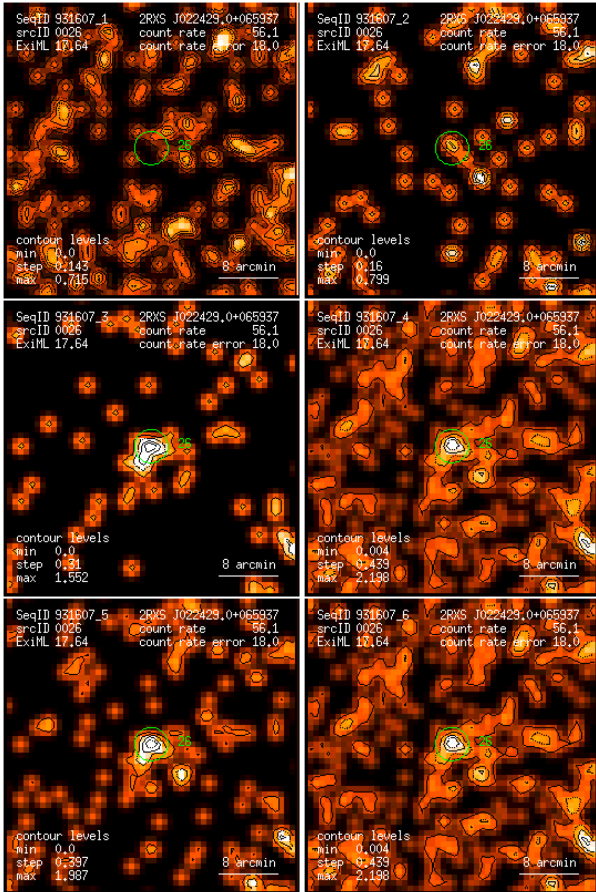
Figure 26: RASS 931607: detection 0026: band rate images, Gaussian filter: (1) PSPC channels 11 – 41, (2) 52 – 90, (3) 91 – 201, (4) 11 – 235, (5) 52 – 201, (6) 11 – 201. Broad band rates in counts/ks. Band rate contour levels in counts/ks/arcmin 2 .
