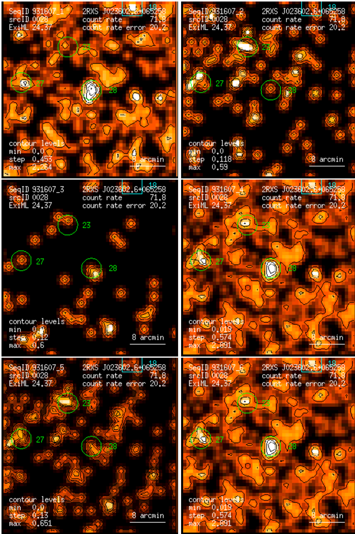
Figure 28: RASS 931607: detection 0028: band rate images, Gaussian filter: (1) PSPC channels 11 – 41, (2) 52 – 90, (3) 91 – 201, (4) 11 – 235, (5) 52 – 201, (6) 11 – 201. Broad band rates in counts/ks. Band rate contour levels in counts/ks/arcmin 2 .
