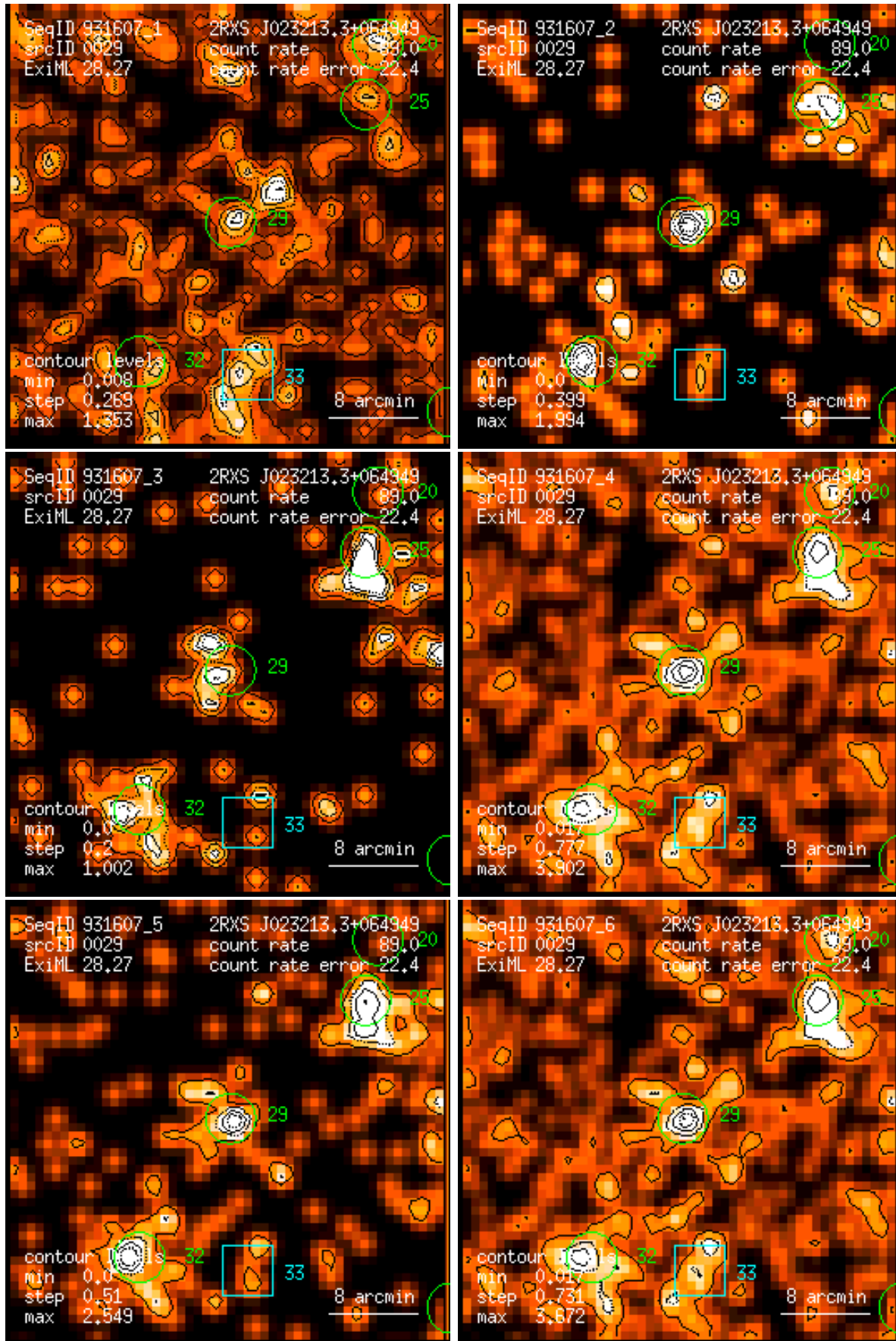
Figure 29: RASS 931607: detection 0029: band rate images, Gaussian filter: (1) PSPC channels 11 – 41, (2) 52 – 90, (3) 91 – 201, (4) 11 – 235, (5) 52 – 201, (6) 11 – 201. Broad band rates in counts/ks. Band rate contour levels in counts/ks/arcmin 2 .
