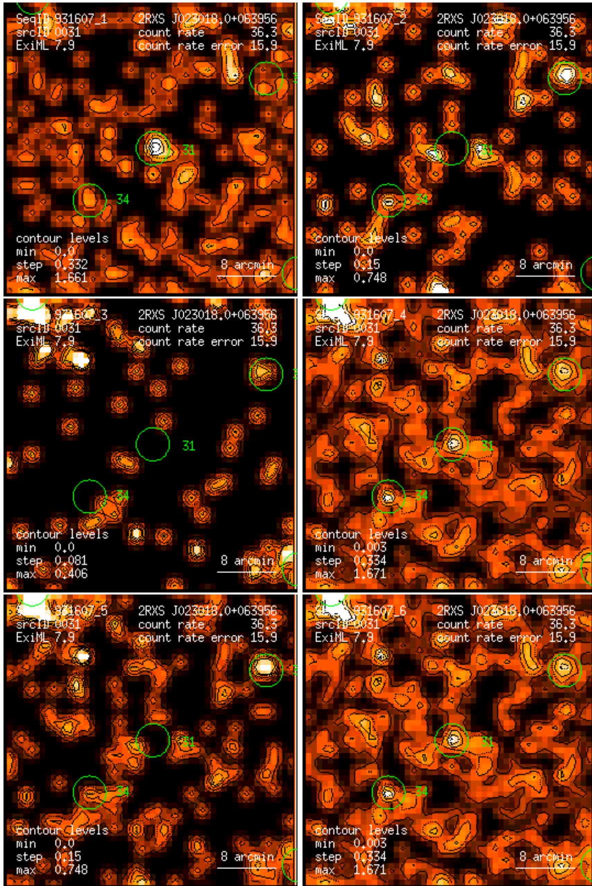
Figure 31: RASS 931607: detection 0031: band rate images, Gaussian filter: (1) PSPC channels 11 – 41, (2) 52 – 90, (3) 91 – 201, (4) 11 – 235, (5) 52 – 201, (6) 11 – 201. Broad band rates in counts/ks. Band rate contour levels in counts/ks/arcmin 2 .
