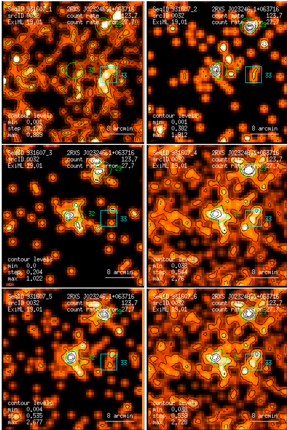
Figure 32: RASS 931607: detection 0032: band rate images, Gaussian filter: (1) PSPC channels 11 – 41, (2) 52 – 90, (3) 91 – 201, (4) 11 – 235, (5) 52 – 201, (6) 11 – 201. Broad band rates in counts/ks. Band rate contour levels in counts/ks/arcmin 2 .
