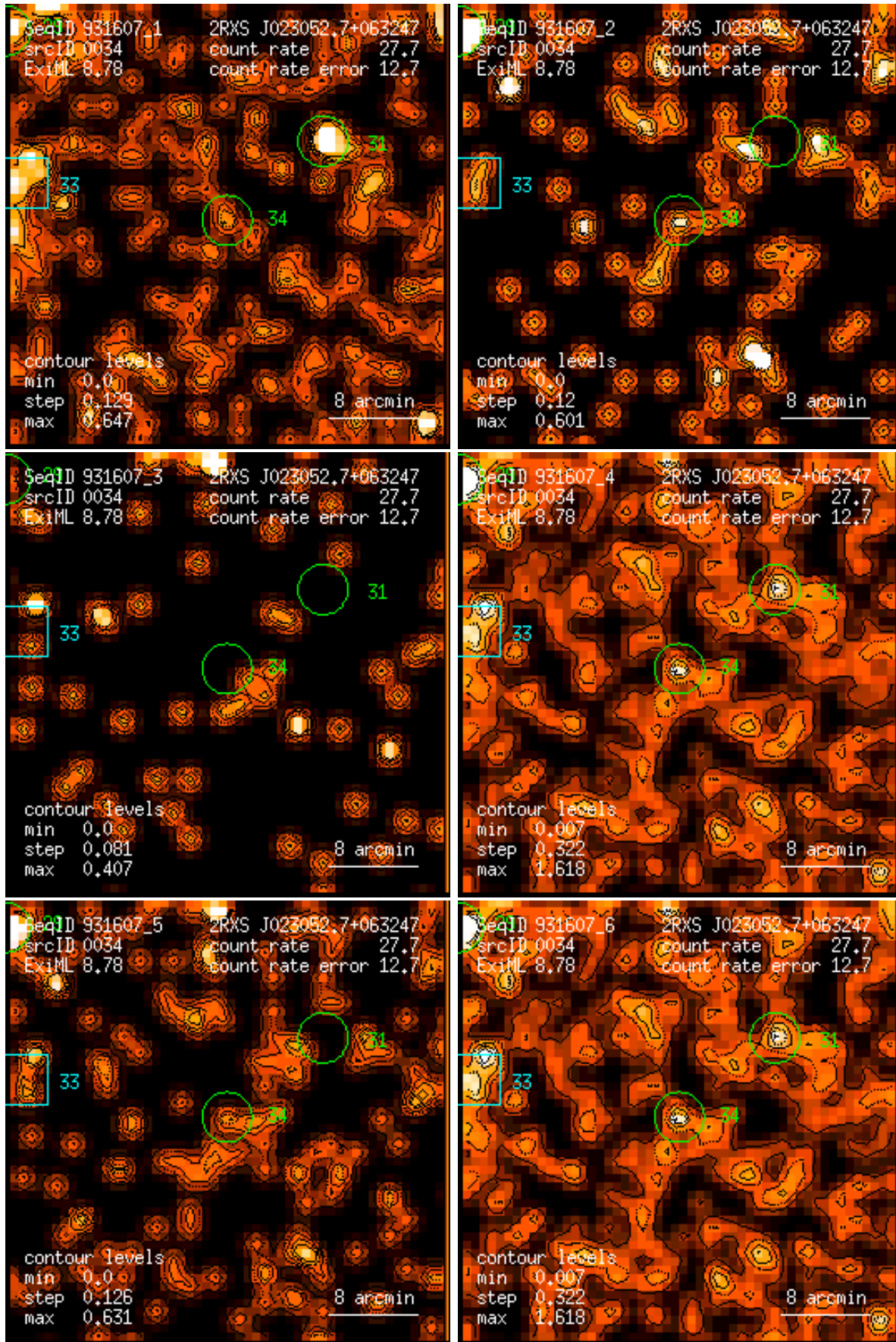
Figure 34: RASS 931607: detection 0034: band rate images, Gaussian filter: (1) PSPC channels 11 – 41, (2) 52 – 90, (3) 91 – 201, (4) 11 – 235, (5) 52 – 201, (6) 11 – 201. Broad band rates in counts/ks. Band rate contour levels in counts/ks/arcmin 2 .
