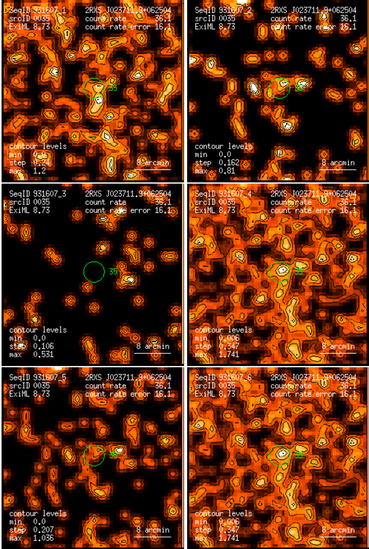
Figure 35: RASS 931607: detection 0035: band rate images, Gaussian filter: (1) PSPC channels 11 – 41, (2) 52 – 90, (3) 91 – 201, (4) 11 – 235, (5) 52 – 201, (6) 11 – 201. Broad band rates in counts/ks. Band rate contour levels in counts/ks/arcmin 2 .
