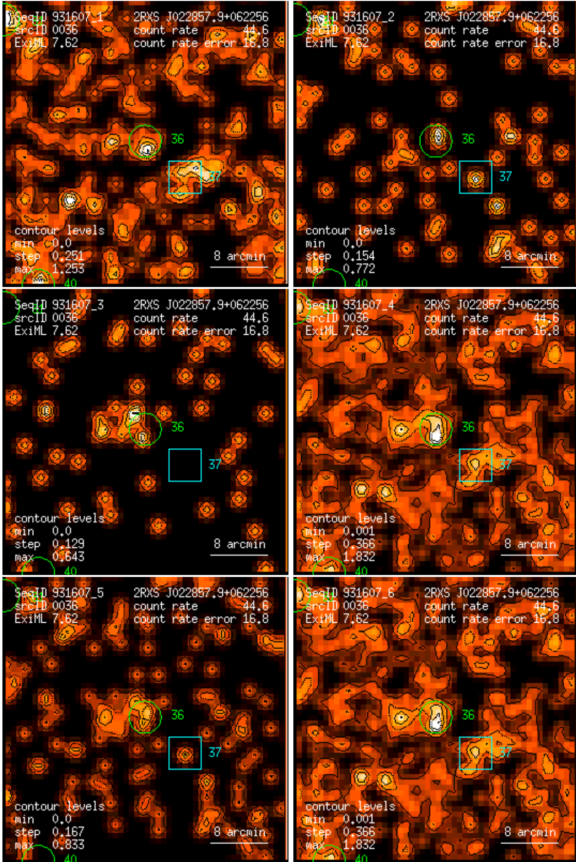
Figure 36: RASS 931607: detection 0036: band rate images, Gaussian filter: (1) PSPC channels 11 – 41, (2) 52 – 90, (3) 91 – 201, (4) 11 – 235, (5) 52 – 201, (6) 11 – 201. Broad band rates in counts/ks. Band rate contour levels in counts/ks/arcmin 2 .
