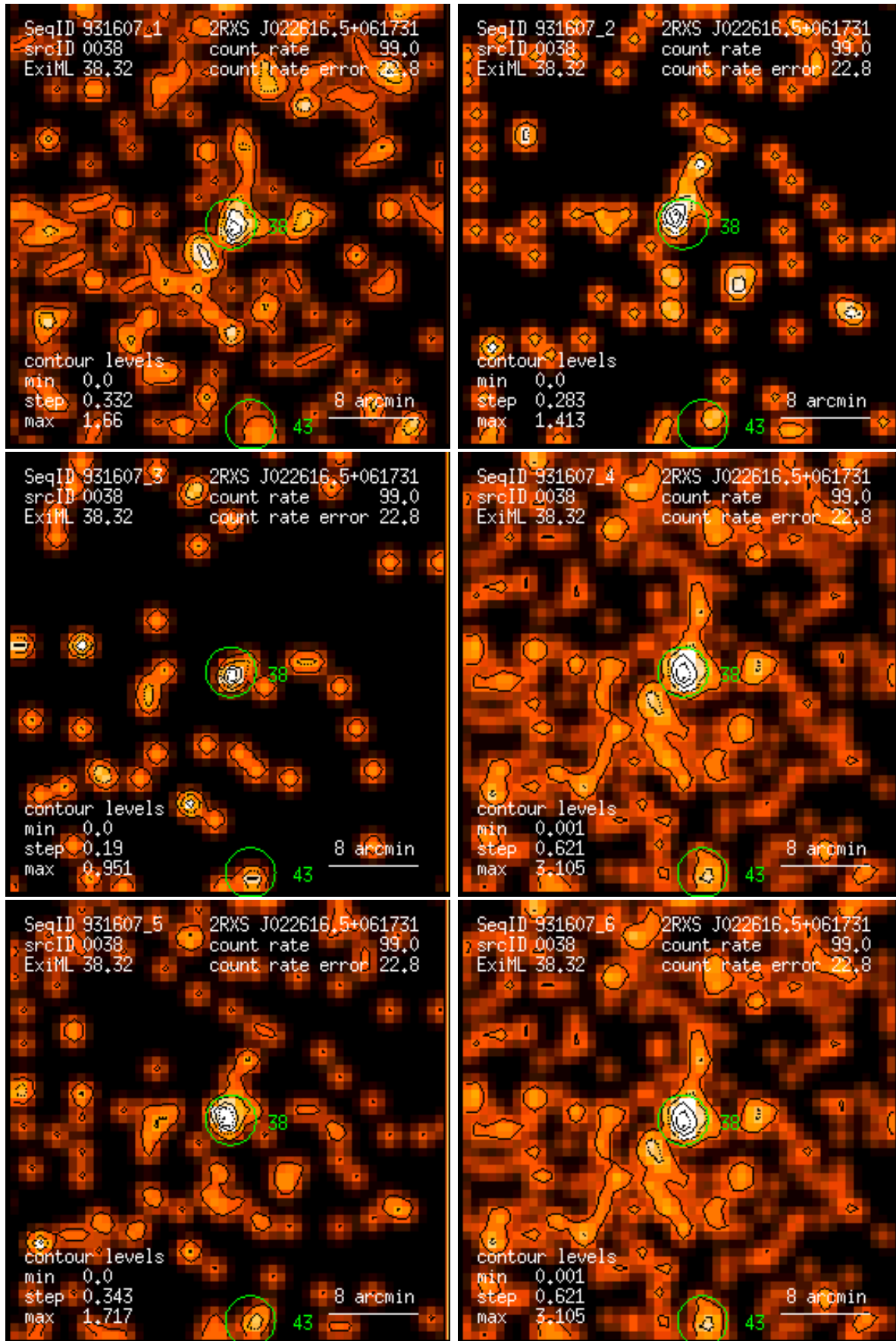
Figure 38: RASS 931607: detection 0038: band rate images, Gaussian filter: (1) PSPC channels 11 – 41, (2) 52 – 90, (3) 91 – 201, (4) 11 – 235, (5) 52 – 201, (6) 11 – 201. Broad band rates in counts/ks. Band rate contour levels in counts/ks/arcmin 2 .
