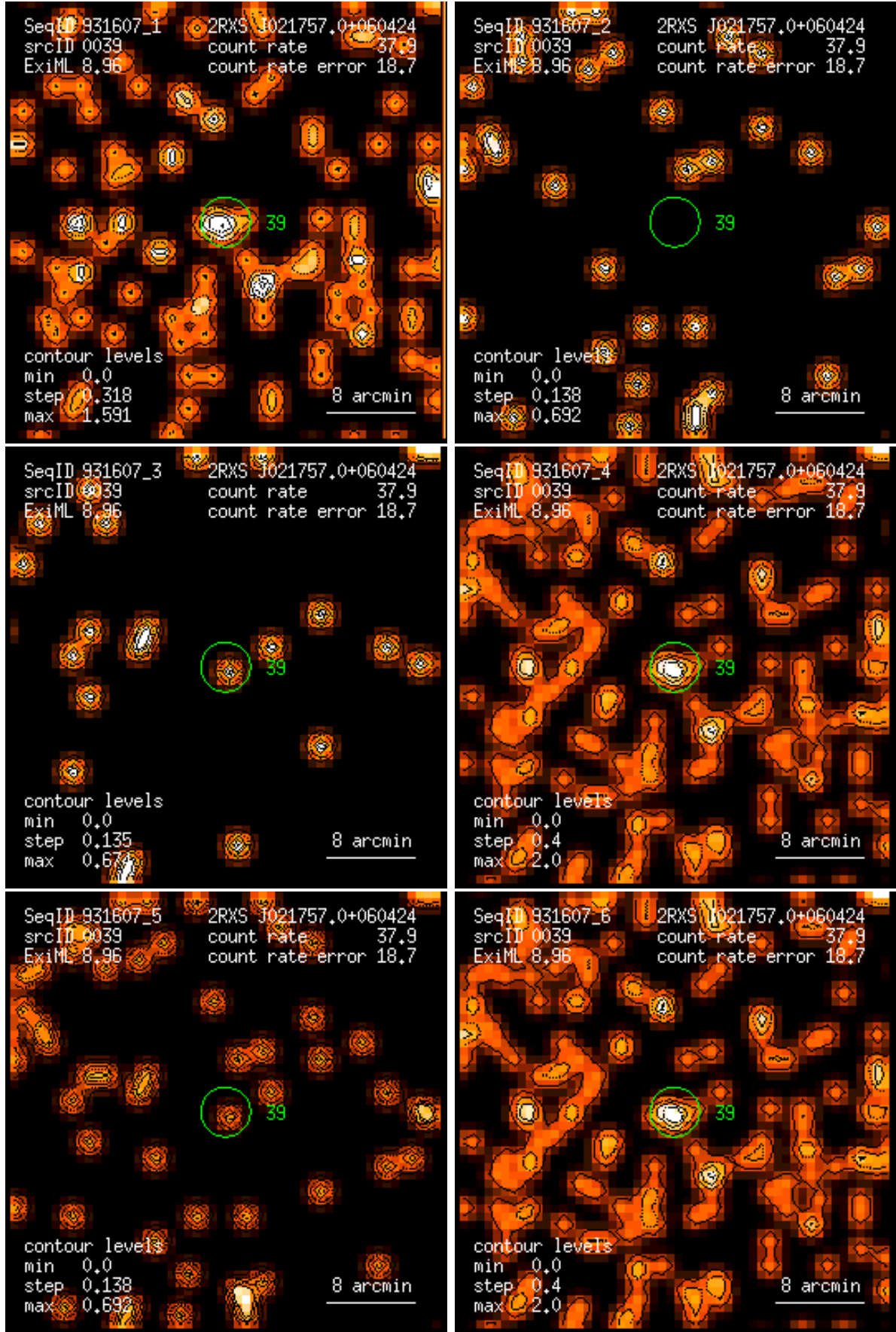
Figure 39: RASS 931607: detection 0039: band rate images, Gaussian filter: (1) PSPC channels 11 – 41, (2) 52 – 90, (3) 91 – 201, (4) 11 – 235, (5) 52 – 201, (6) 11 – 201. Broad band rates in counts/ks. Band rate contour levels in counts/ks/arcmin 2 .
