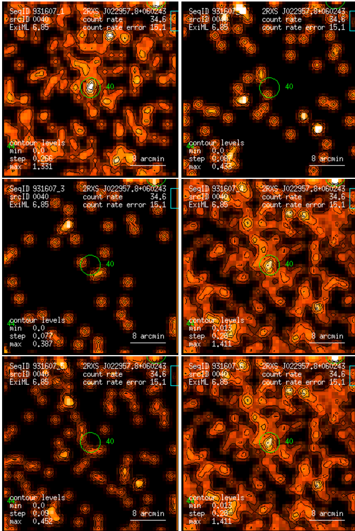
Figure 40: RASS 931607: detection 0040: band rate images, Gaussian filter: (1) PSPC channels 11 – 41, (2) 52 – 90, (3) 91 – 201, (4) 11 – 235, (5) 52 – 201, (6) 11 – 201. Broad band rates in counts/ks. Band rate contour levels in counts/ks/arcmin 2 .
