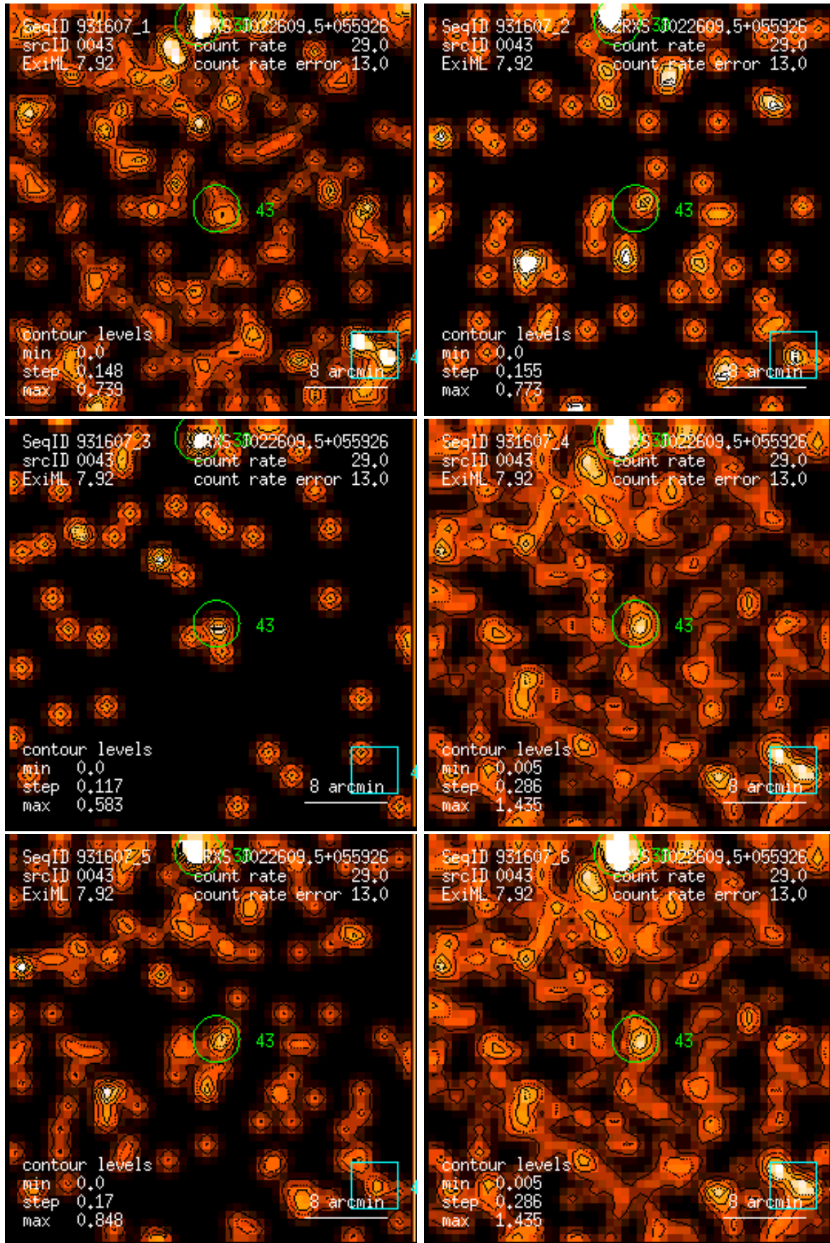
Figure 43: RASS 931607: detection 0043: band rate images, Gaussian filter: (1) PSPC channels 11 – 41, (2) 52 – 90, (3) 91 – 201, (4) 11 – 235, (5) 52 – 201, (6) 11 – 201. Broad band rates in counts/ks. Band rate contour levels in counts/ks/arcmin 2 .
