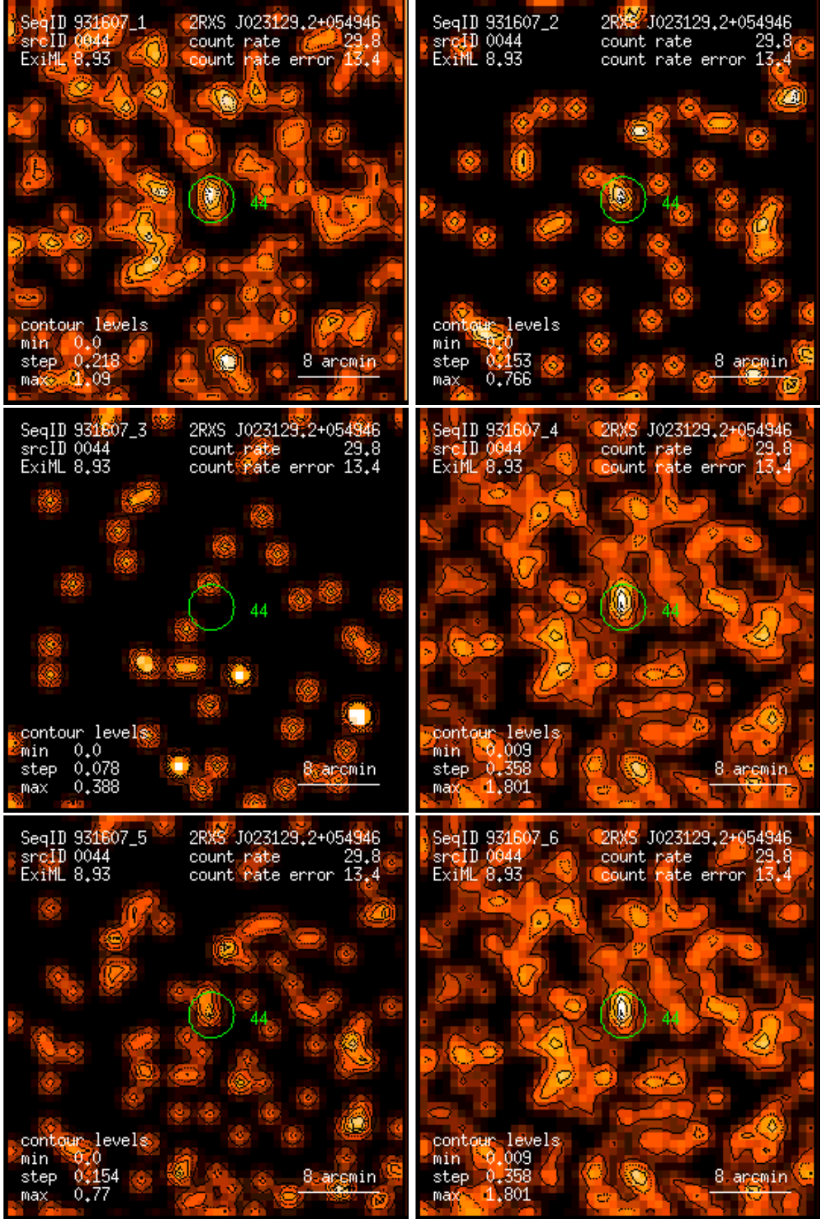
Figure 44: RASS 931607: detection 0044: band rate images, Gaussian filter: (1) PSPC channels 11 – 41, (2) 52 – 90, (3) 91 – 201, (4) 11 – 235, (5) 52 – 201, (6) 11 – 201. Broad band rates in counts/ks. Band rate contour levels in counts/ks/arcmin 2 .
