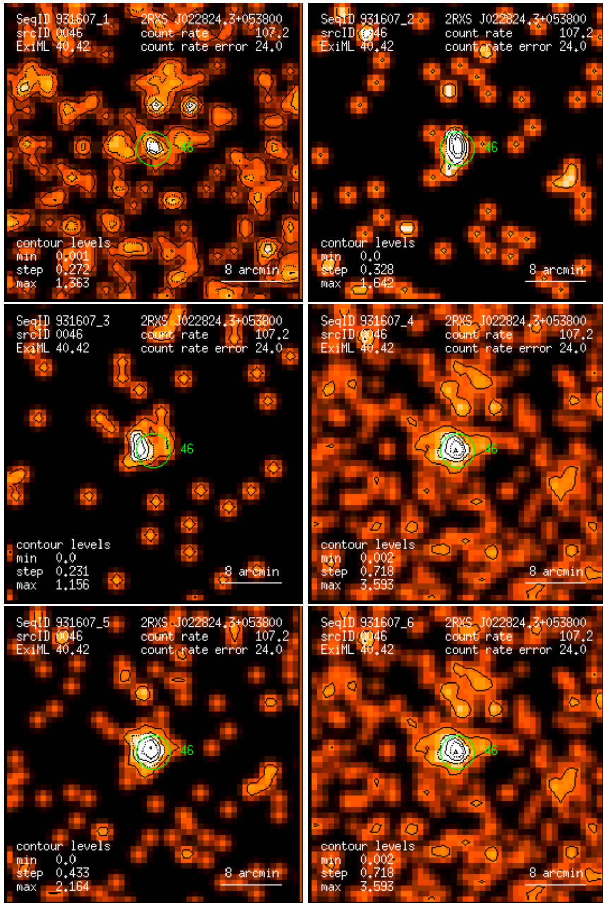
Figure 46: RASS 931607: detection 0046: band rate images, Gaussian filter: (1) PSPC channels 11 – 41, (2) 52 – 90, (3) 91 – 201, (4) 11 – 235, (5) 52 – 201, (6) 11 – 201. Broad band rates in counts/ks. Band rate contour levels in counts/ks/arcmin 2 .
