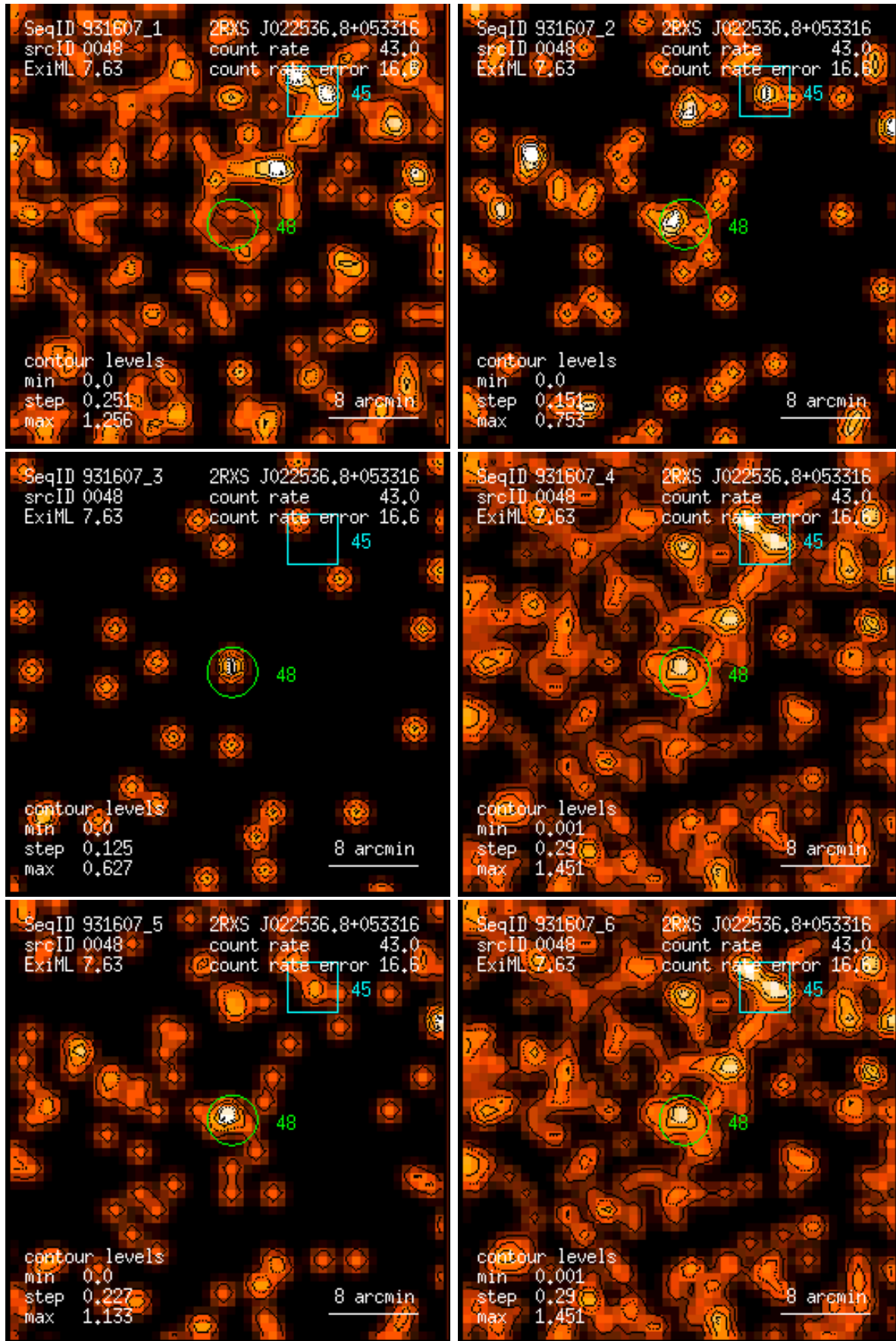
Figure 48: RASS 931607: detection 0048: band rate images, Gaussian filter: (1) PSPC channels 11 – 41, (2) 52 – 90, (3) 91 – 201, (4) 11 – 235, (5) 52 – 201, (6) 11 – 201. Broad band rates in counts/ks. Band rate contour levels in counts/ks/arcmin 2 .
