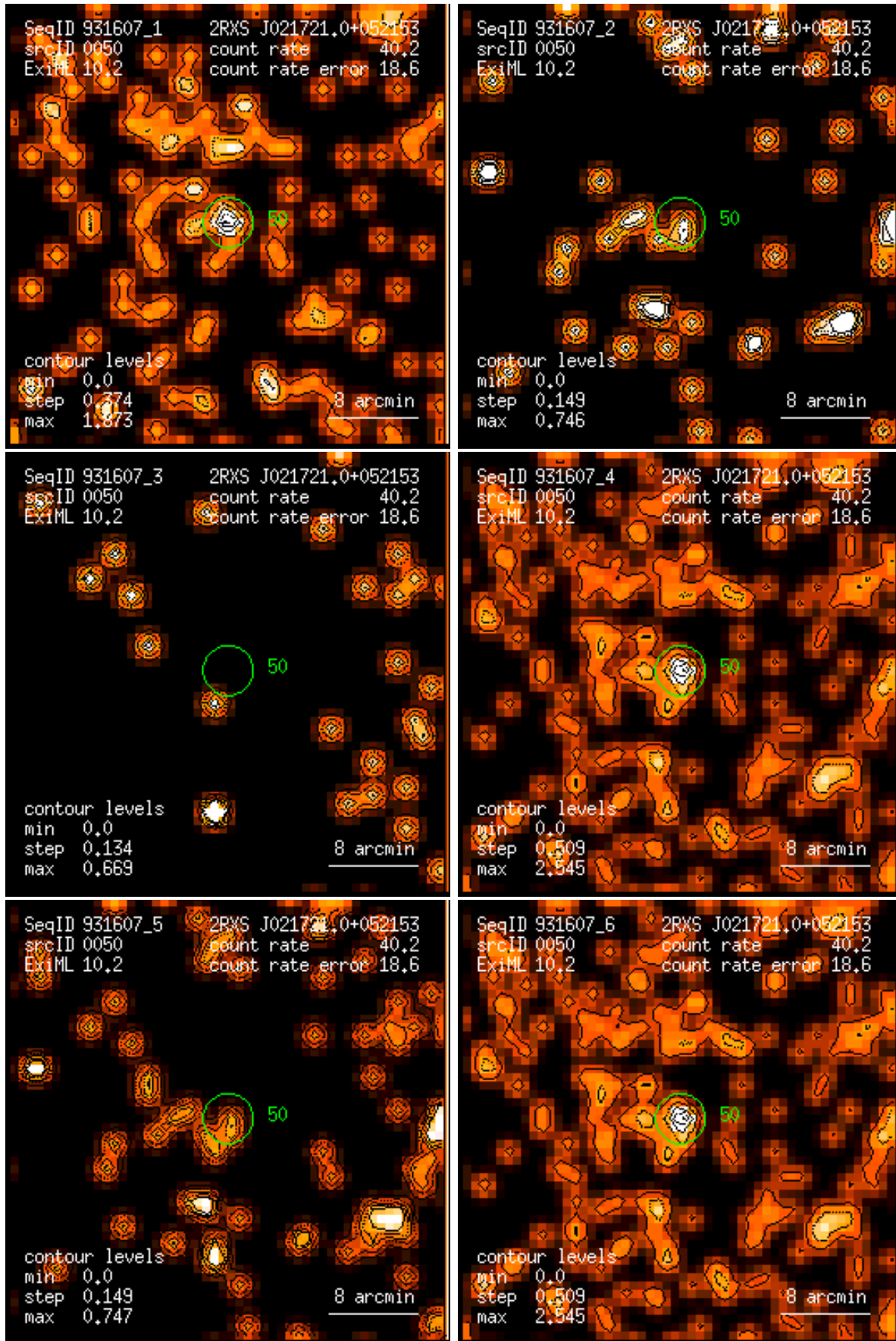
Figure 50: RASS 931607: detection 0050: band rate images, Gaussian filter: (1) PSPC channels 11 – 41, (2) 52 – 90, (3) 91 – 201, (4) 11 – 235, (5) 52 – 201, (6) 11 – 201. Broad band rates in counts/ks. Band rate contour levels in counts/ks/arcmin 2 .
