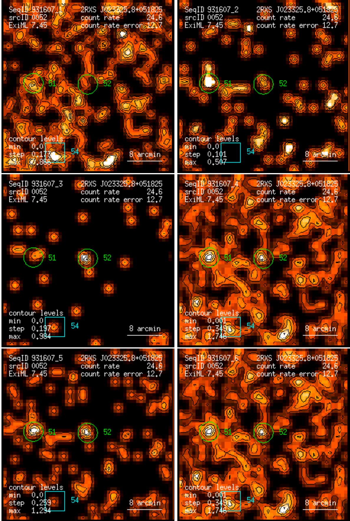
Figure 52: RASS 931607: detection 0052: band rate images, Gaussian filter: (1) PSPC channels 11 – 41, (2) 52 – 90, (3) 91 – 201, (4) 11 – 235, (5) 52 – 201, (6) 11 – 201. Broad band rates in counts/ks. Band rate contour levels in counts/ks/arcmin 2 .
