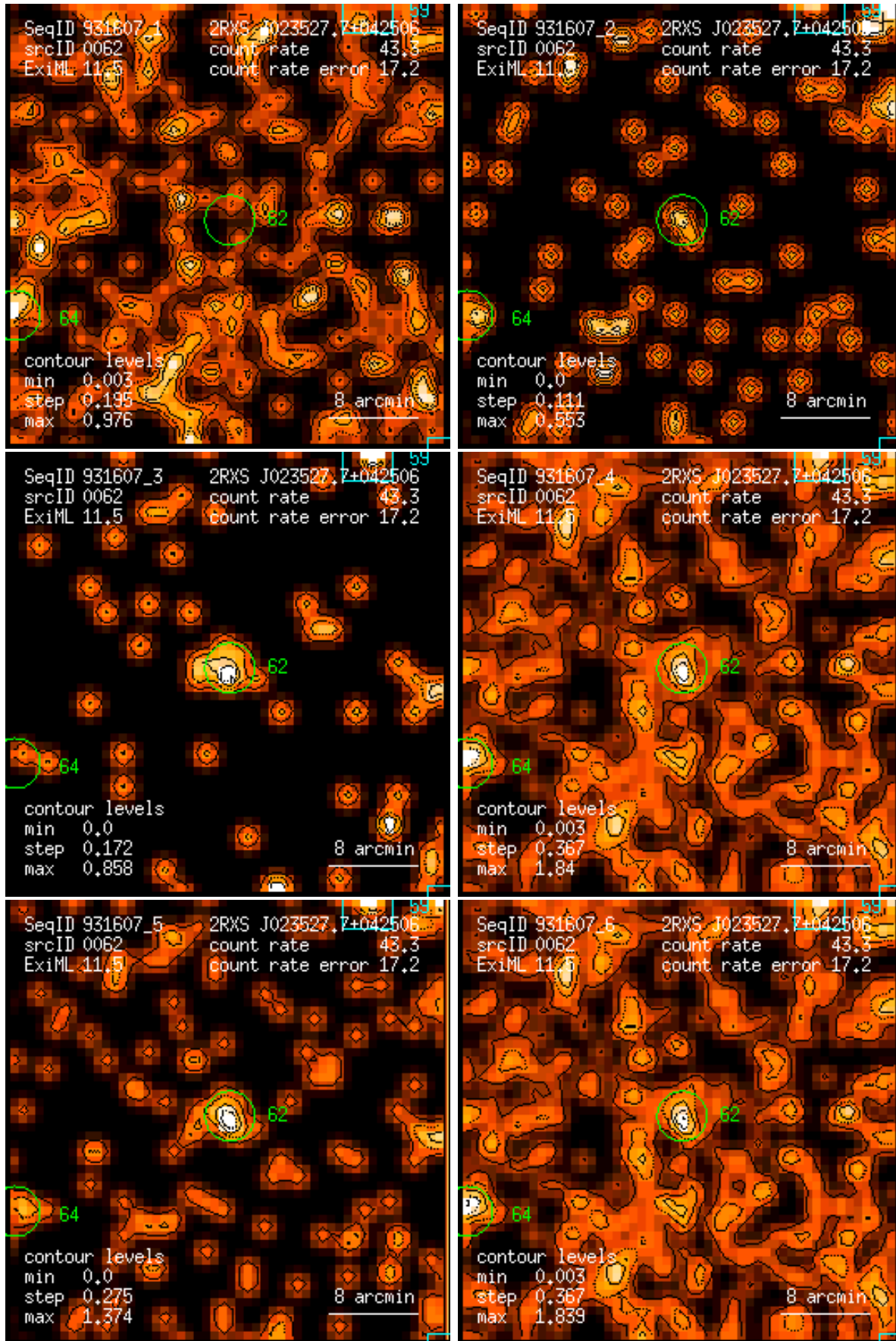
Figure 62: RASS 931607: detection 0062: band rate images, Gaussian filter: (1) PSPC channels 11 – 41, (2) 52 – 90, (3) 91 – 201, (4) 11 – 235, (5) 52 – 201, (6) 11 – 201. Broad band rates in counts/ks. Band rate contour levels in counts/ks/arcmin 2 .
