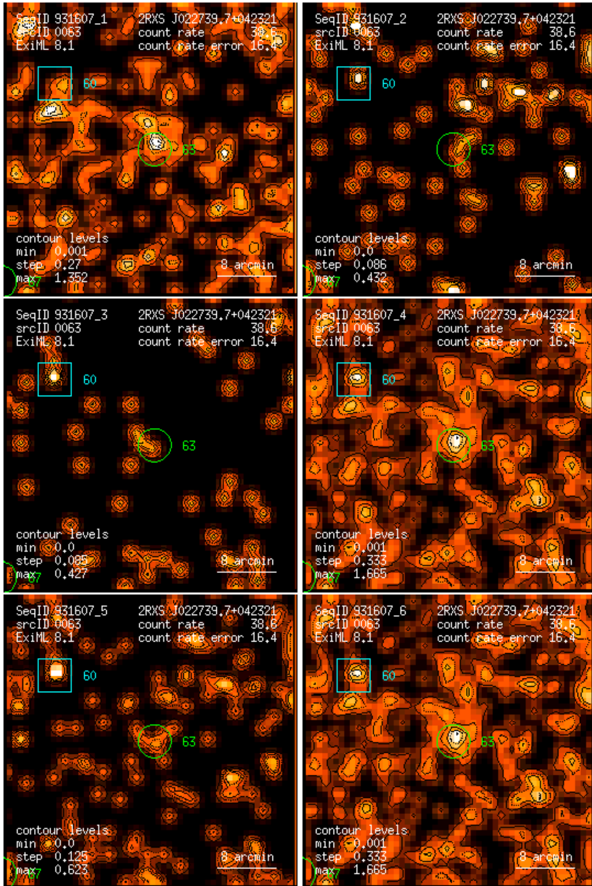
Figure 63: RASS 931607: detection 0063: band rate images, Gaussian filter: (1) PSPC channels 11 – 41, (2) 52 – 90, (3) 91 – 201, (4) 11 – 235, (5) 52 – 201, (6) 11 – 201. Broad band rates in counts/ks. Band rate contour levels in counts/ks/arcmin 2 .
