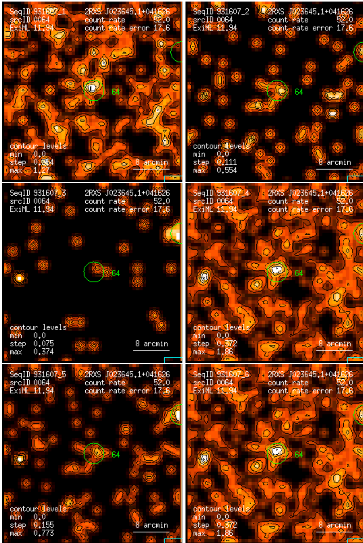
Figure 64: RASS 931607: detection 0064: band rate images, Gaussian filter: (1) PSPC channels 11 – 41, (2) 52 – 90, (3) 91 – 201, (4) 11 – 235, (5) 52 – 201, (6) 11 – 201. Broad band rates in counts/ks. Band rate contour levels in counts/ks/arcmin 2 .
