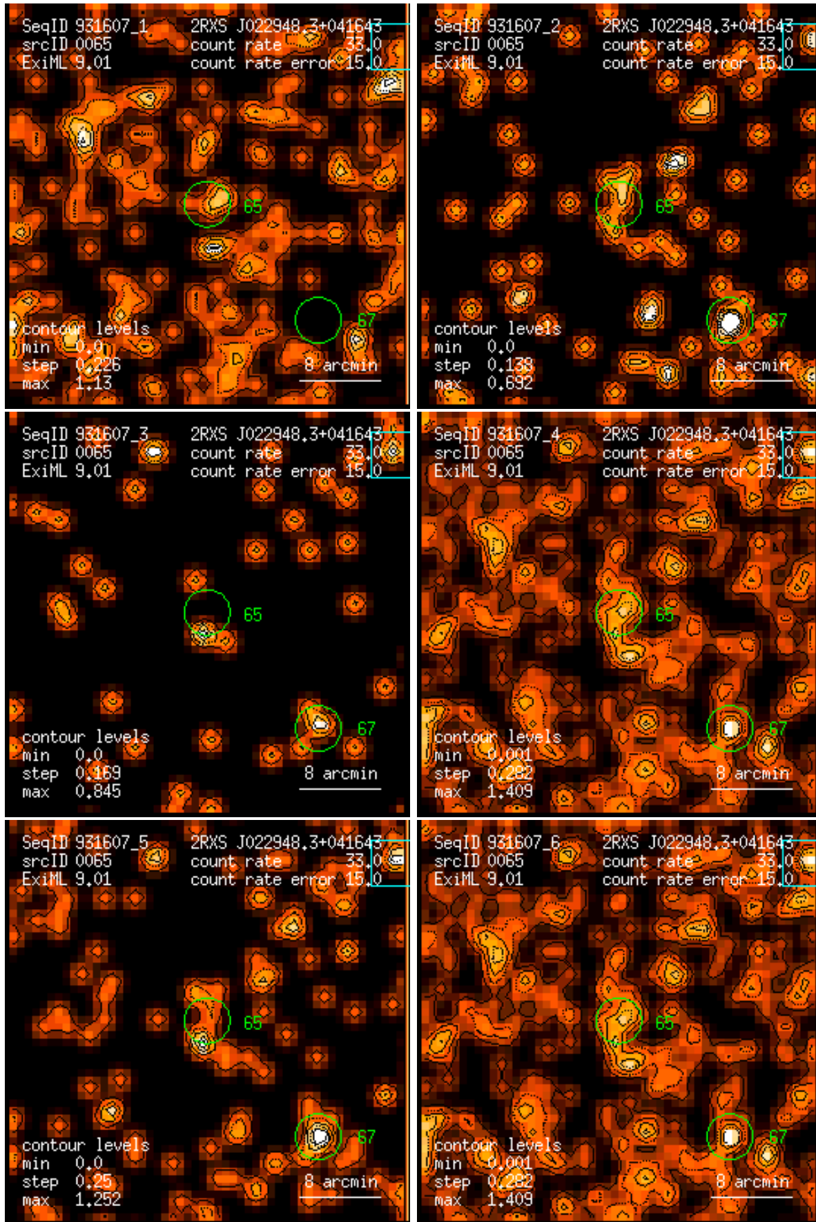
Figure 65: RASS 931607: detection 0065: band rate images, Gaussian filter: (1) PSPC channels 11 – 41, (2) 52 – 90, (3) 91 – 201, (4) 11 – 235, (5) 52 – 201, (6) 11 – 201. Broad band rates in counts/ks. Band rate contour levels in counts/ks/arcmin 2 .
