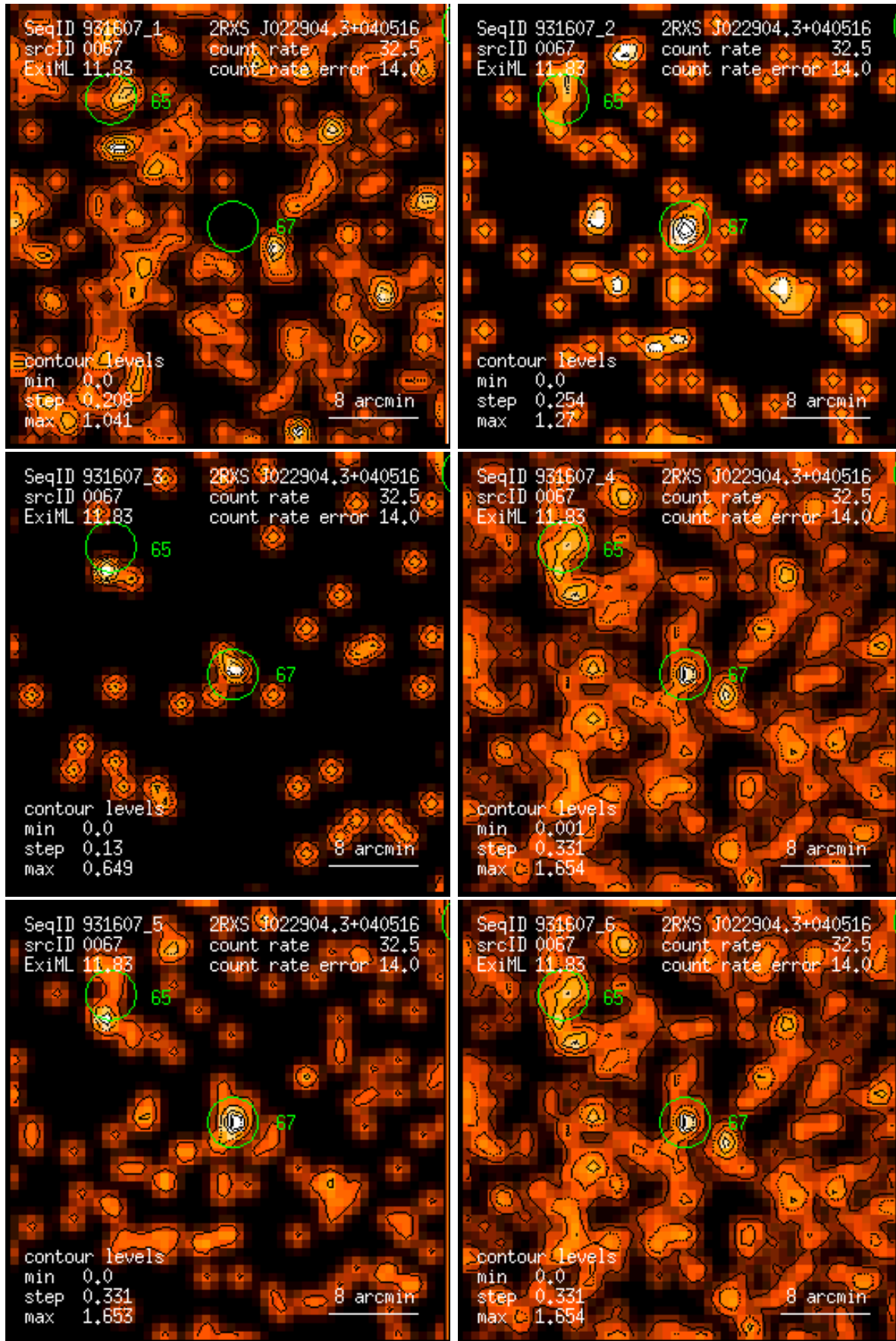
Figure 67: RASS 931607: detection 0067: band rate images, Gaussian filter: (1) PSPC channels 11 – 41, (2) 52 – 90, (3) 91 – 201, (4) 11 – 235, (5) 52 – 201, (6) 11 – 201. Broad band rates in counts/ks. Band rate contour levels in counts/ks/arcmin 2 .
