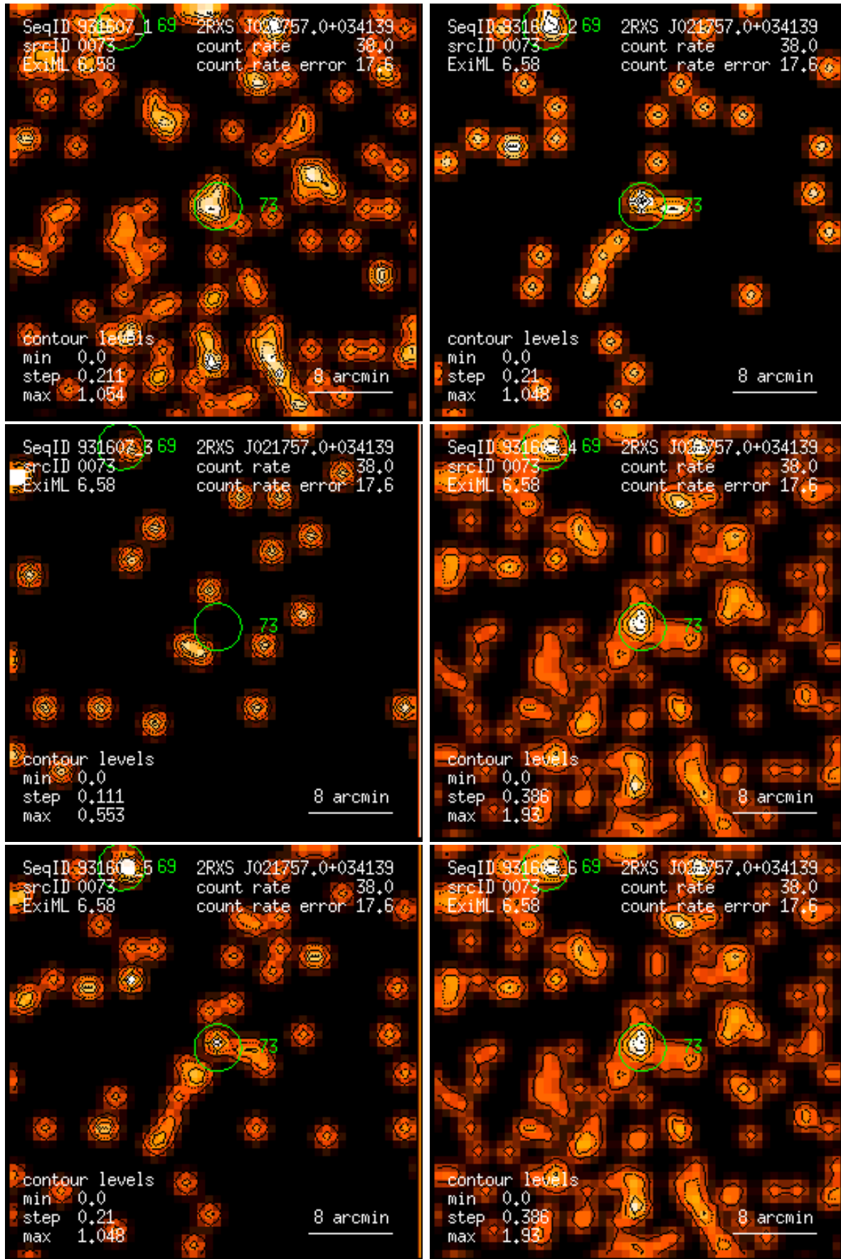
Figure 73: RASS 931607: detection 0073: band rate images, Gaussian filter: (1) PSPC channels 11 – 41, (2) 52 – 90, (3) 91 – 201, (4) 11 – 235, (5) 52 – 201, (6) 11 – 201. Broad band rates in counts/ks. Band rate contour levels in counts/ks/arcmin 2 .
