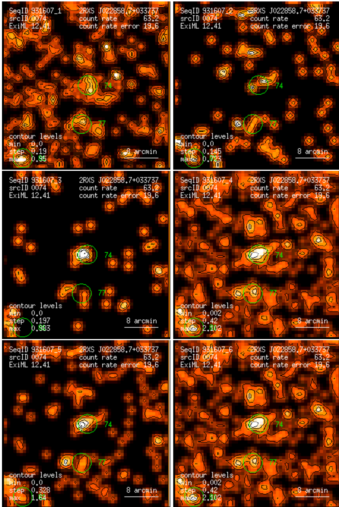
Figure 74: RASS 931607: detection 0074: band rate images, Gaussian filter: (1) PSPC channels 11 – 41, (2) 52 – 90, (3) 91 – 201, (4) 11 – 235, (5) 52 – 201, (6) 11 – 201. Broad band rates in counts/ks. Band rate contour levels in counts/ks/arcmin 2 .
