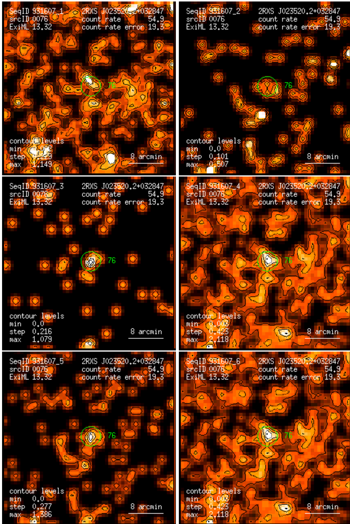
Figure 76: RASS 931607: detection 0076: band rate images, Gaussian filter: (1) PSPC channels 11 – 41, (2) 52 – 90, (3) 91 – 201, (4) 11 – 235, (5) 52 – 201, (6) 11 – 201. Broad band rates in counts/ks. Band rate contour levels in counts/ks/arcmin 2 .
