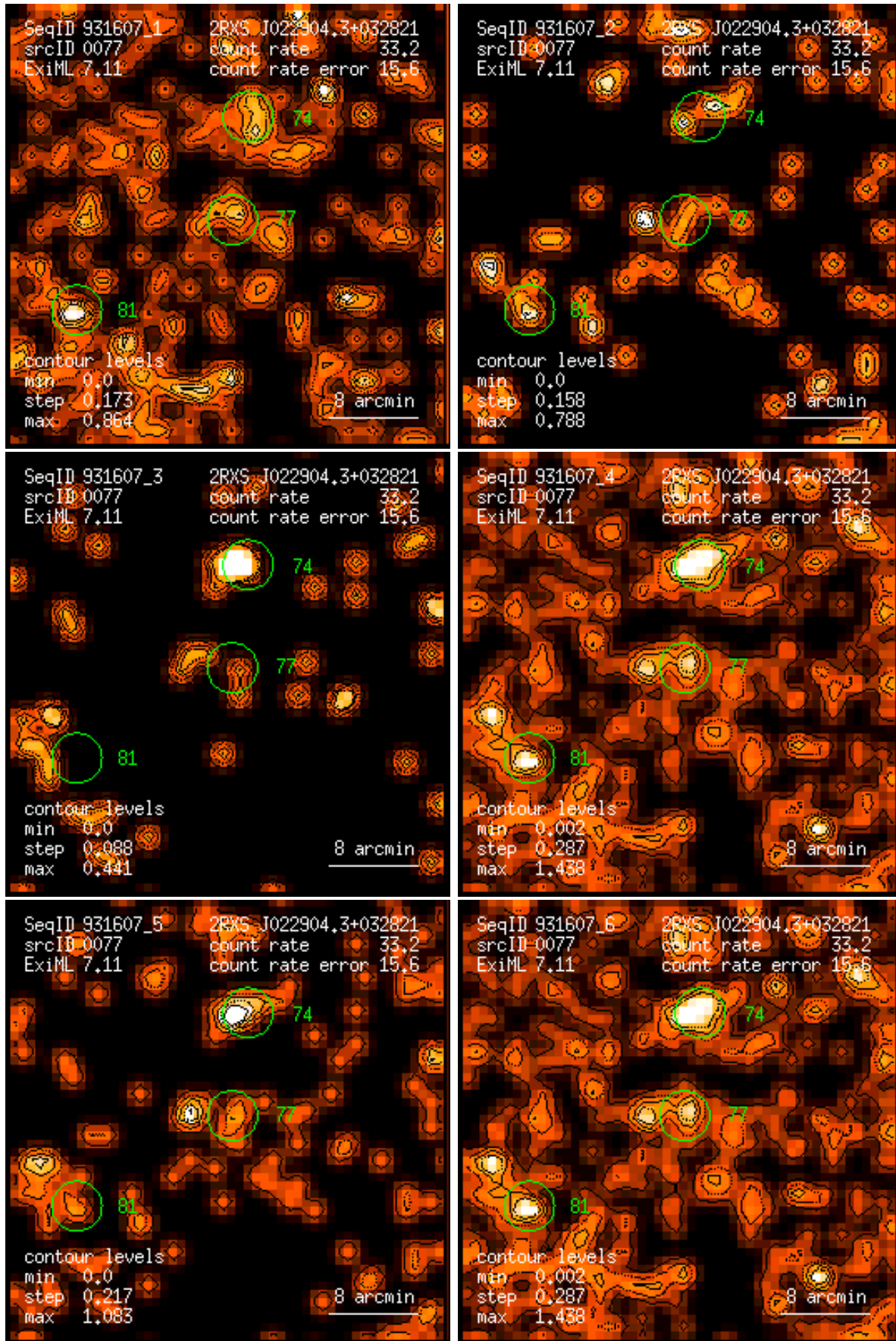
Figure 77: RASS 931607: detection 0077: band rate images, Gaussian filter: (1) PSPC channels 11 – 41, (2) 52 – 90, (3) 91 – 201, (4) 11 – 235, (5) 52 – 201, (6) 11 – 201. Broad band rates in counts/ks. Band rate contour levels in counts/ks/arcmin 2 .
