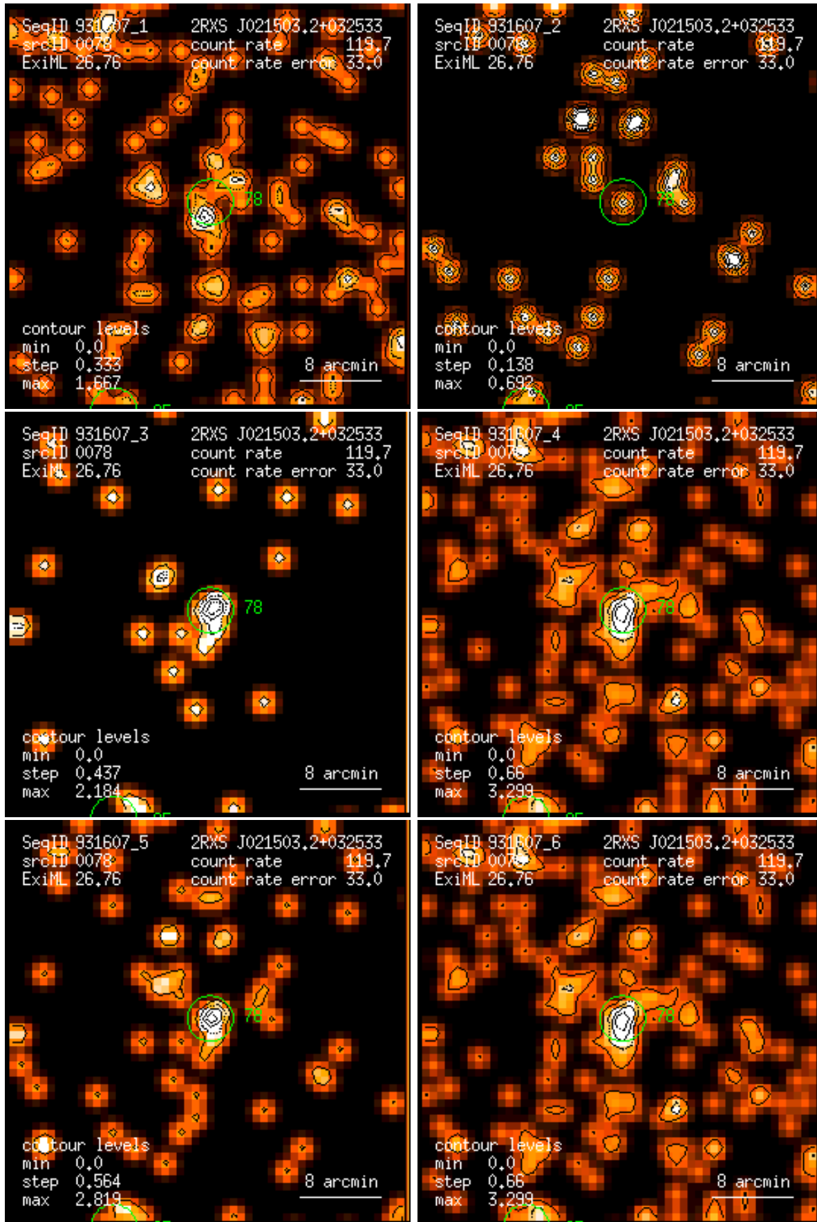
Figure 78: RASS 931607: detection 0078: band rate images, Gaussian filter: (1) PSPC channels 11 – 41, (2) 52 – 90, (3) 91 – 201, (4) 11 – 235, (5) 52 – 201, (6) 11 – 201. Broad band rates in counts/ks. Band rate contour levels in counts/ks/arcmin 2 .
