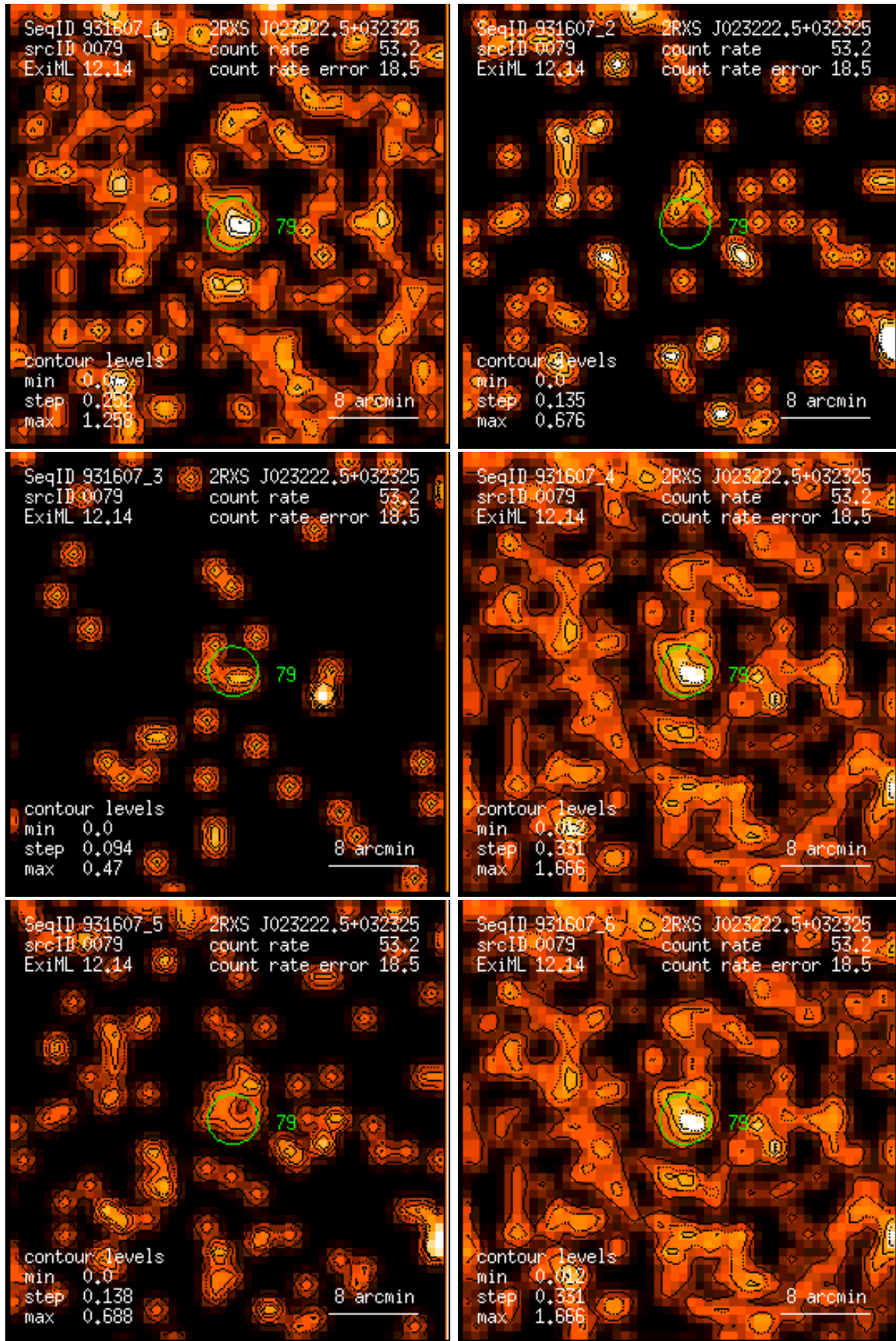
Figure 79: RASS 931607: detection 0079: band rate images, Gaussian filter: (1) PSPC channels 11 – 41, (2) 52 – 90, (3) 91 – 201, (4) 11 – 235, (5) 52 – 201, (6) 11 – 201. Broad band rates in counts/ks. Band rate contour levels in counts/ks/arcmin 2 .
