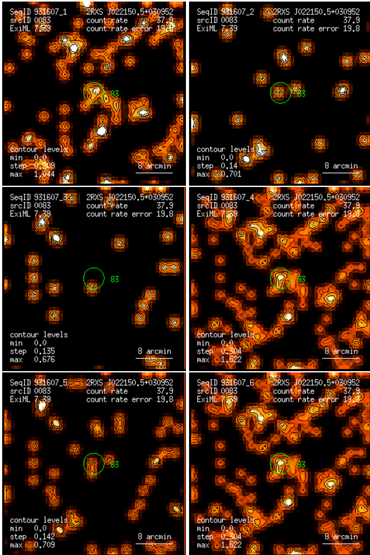
Figure 83: RASS 931607: detection 0083: band rate images, Gaussian filter: (1) PSPC channels 11 – 41, (2) 52 – 90, (3) 91 – 201, (4) 11 – 235, (5) 52 – 201, (6) 11 – 201. Broad band rates in counts/ks. Band rate contour levels in counts/ks/arcmin 2 .
