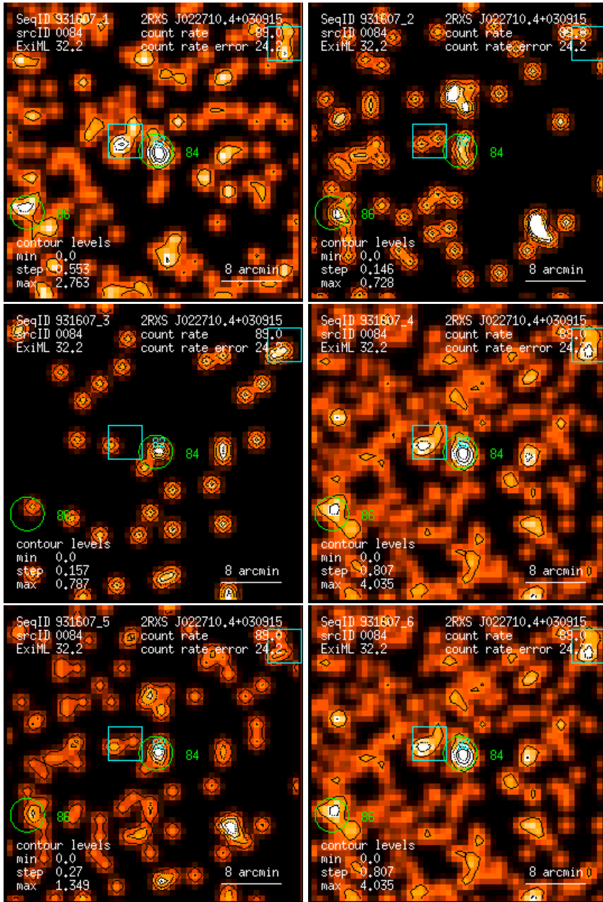
Figure 84: RASS 931607: detection 0084: band rate images, Gaussian filter: (1) PSPC channels 11 – 41, (2) 52 – 90, (3) 91 – 201, (4) 11 – 235, (5) 52 – 201, (6) 11 – 201. Broad band rates in counts/ks. Band rate contour levels in counts/ks/arcmin 2 .
