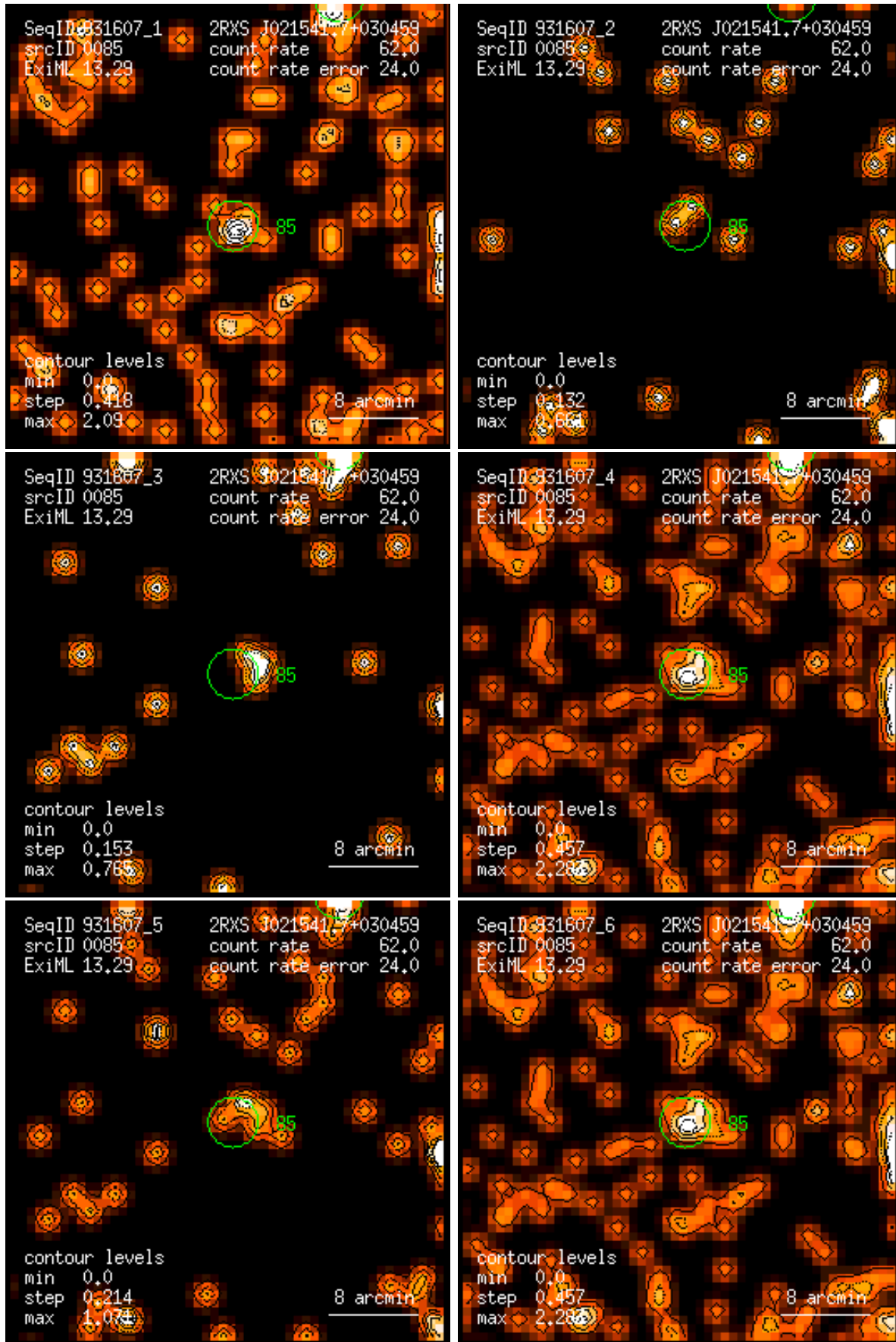
Figure 85: RASS 931607: detection 0085: band rate images, Gaussian filter: (1) PSPC channels 11 – 41, (2) 52 – 90, (3) 91 – 201, (4) 11 – 235, (5) 52 – 201, (6) 11 – 201. Broad band rates in counts/ks. Band rate contour levels in counts/ks/arcmin 2 .
