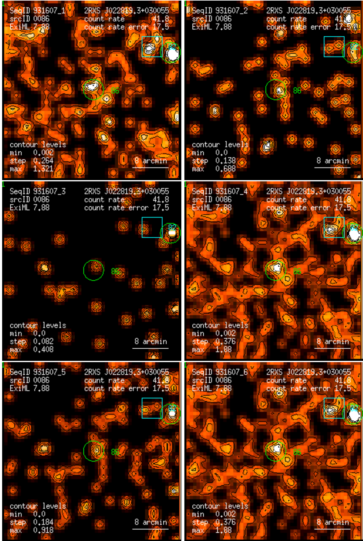
Figure 86: RASS 931607: detection 0086: band rate images, Gaussian filter: (1) PSPC channels 11 – 41, (2) 52 – 90, (3) 91 – 201, (4) 11 – 235, (5) 52 – 201, (6) 11 – 201. Broad band rates in counts/ks. Band rate contour levels in counts/ks/arcmin 2 .
